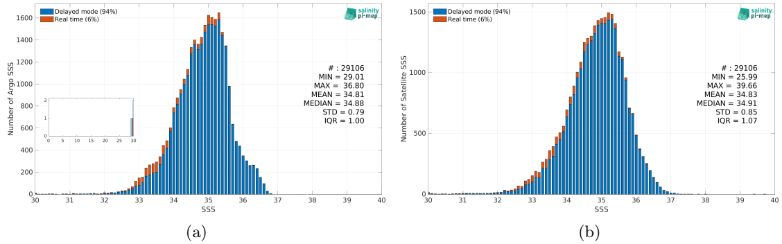
Figure 2: Histograms of SSS from Argo (a) and Aquarius SSS L2 CAP v5 (JPL) (b) considering all match-up pairs per bins of 0.1 over the Tropical Pacific Ocean Pi-MEP region and for the full satellite product period.
