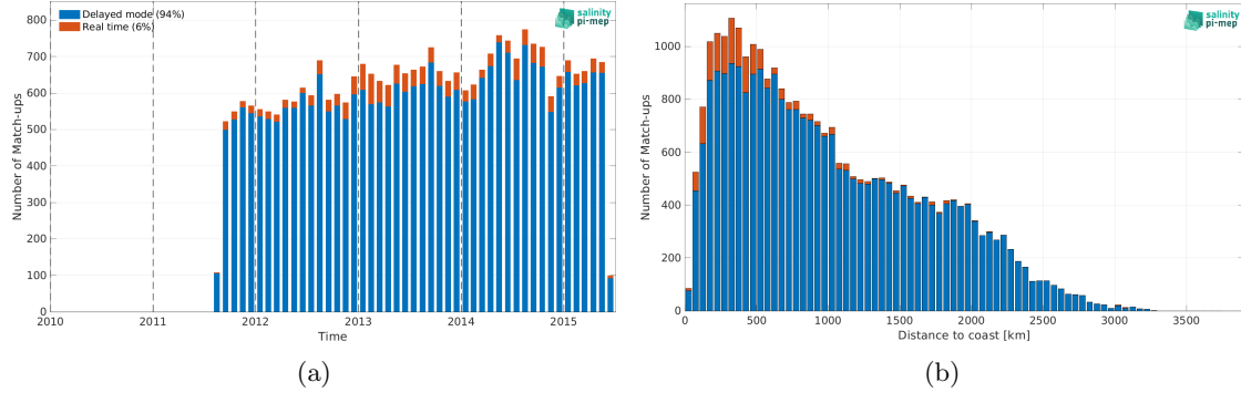
Figure 1: Number of match-ups between Argo and Aquarius SSS L2 CAP v5 (JPL) SSS as a function of time (a) and as function of the distance to coast (b) over the Tropical Pacific Ocean Pi-MEP region and for the full satellite product period.
