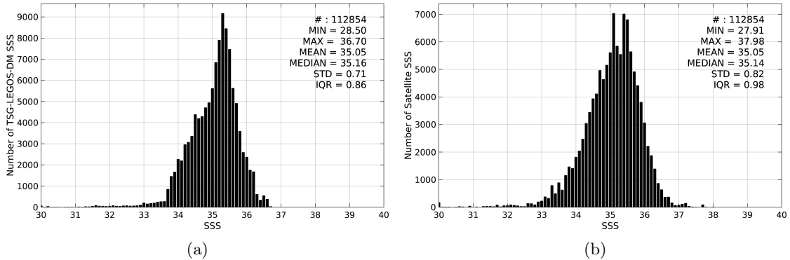
Figure 2: Histograms of SSS from TSG-LEGOS-DM (a) and AQUARIUS-L2-JPL-V4 (b) considering all match-up pairs per bins of 0.1 over the Tropical Pacific Ocean Pi-MEP region and for the full satellite product period.
