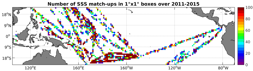
Figure 4: Number of SSS match-ups between TSG-LEGOS-DM SSS and the AQUARIUS-L2-JPL-V4 SSS product for the Tropical Pacific Ocean Pi-MEP region over 1^\circ \times 1^\circ boxes and for the full satellite product period.
