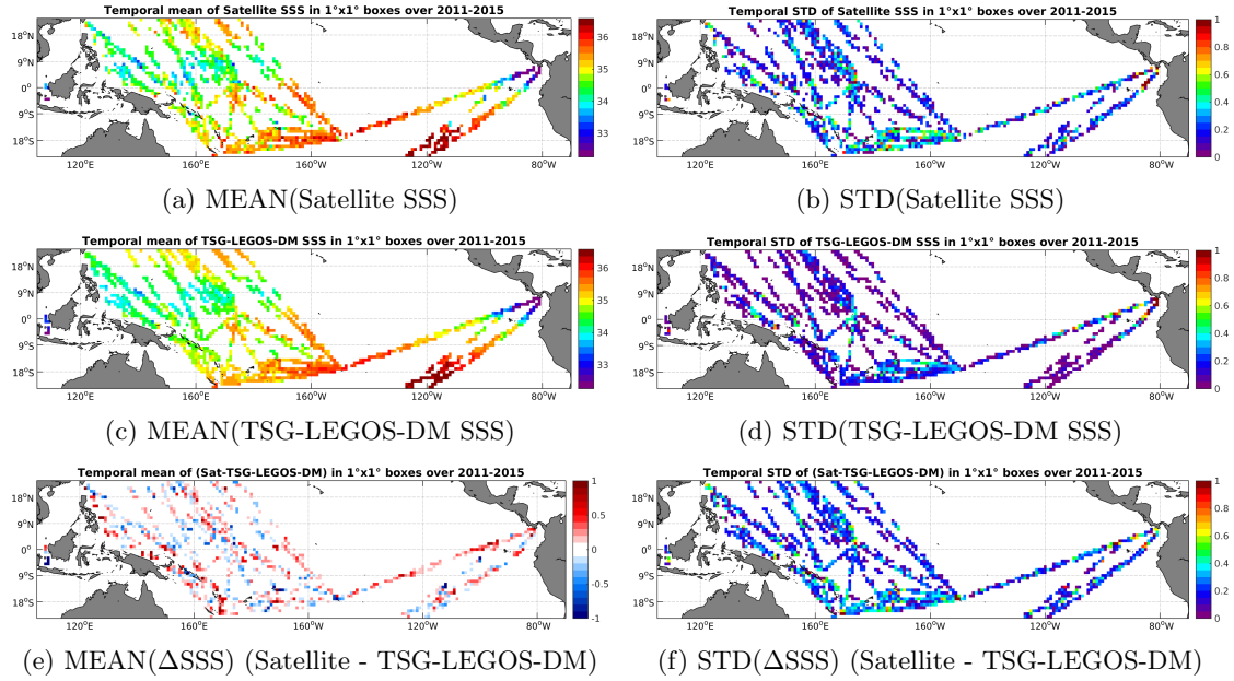
Figure 6: Temporal mean (left) and STD (right) of SSS from AQUARIUS-L2-JPL-V4 (top), TSG-LEGOS-DM (middle), and of \Delta SSS (Satellite - TSG-LEGOS-DM). Only match-up pairs are used to generate these maps.
