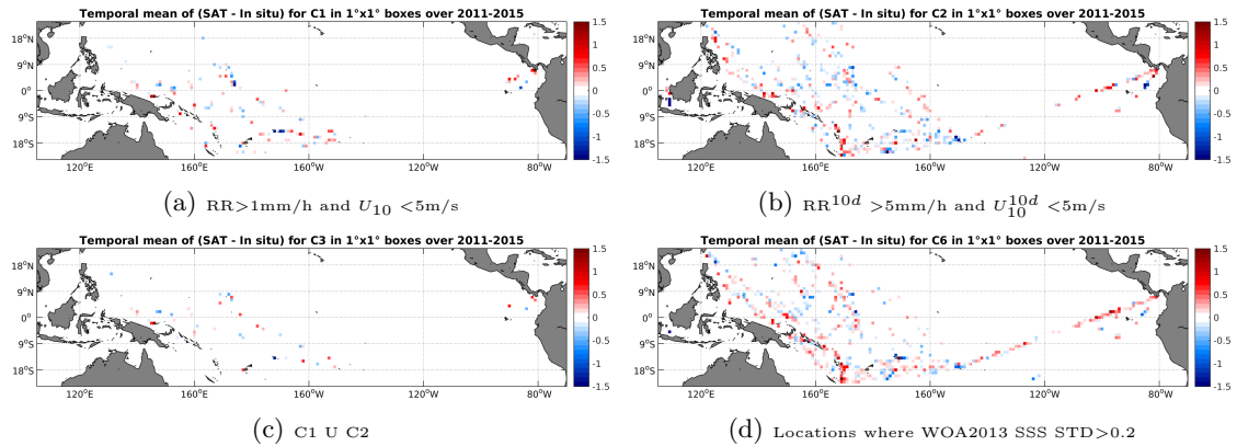
Figure 12: Temporal mean gridded over spatial boxes of size 1^\circ \times 1^\circ of \Delta SSS (AQUARIUS-L2-JPL-V4 - TSG-LEGOS-DM) for 4 different subdatasets corresponding to: RR > 1\text{mm/h} and U_{10} < 5\text{m/s} (a), RR^{10d} > 5\text{mm/h} and U_{10}^{10d} < 5\text{m/s} (b), C1 U C2 (c), Locations where WOA2013 SSS STD > 0.2 (d).
