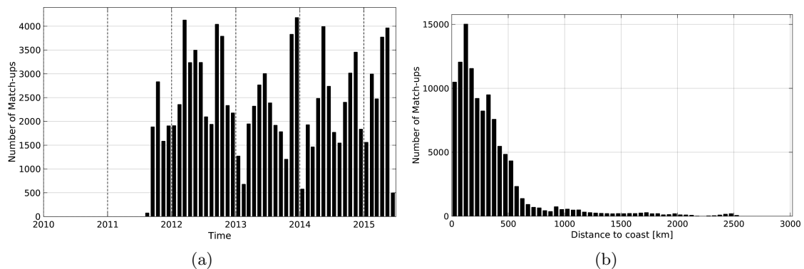
Figure 1: Number of match-ups between TSG-LEGOS-DM and AQUARIUS-L2-JPL-V4 SSS as a function of time (a) and as function of the distance to coast (b) over the Tropical Pacific Ocean Pi-MEP region and for the full satellite product period.
