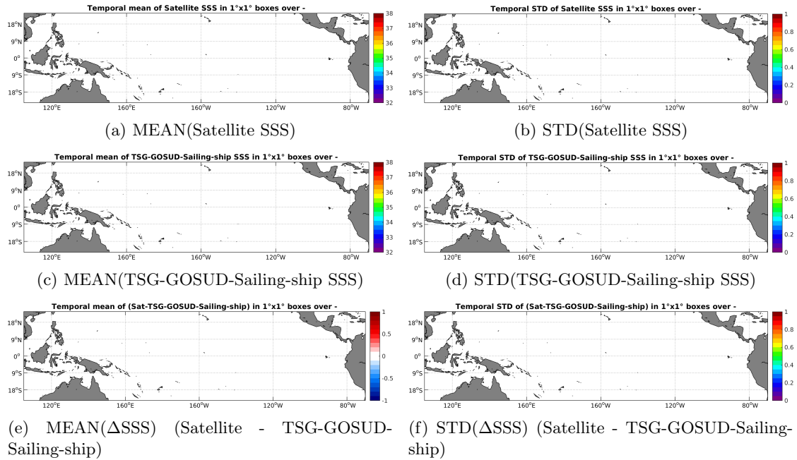
Figure 6: Temporal mean (left) and STD (right) of SSS from AQUARIUS-L2-JPL-V4 (top), TSG-GOSUD-Sailing-ship (middle), and of \Delta SSS (Satellite - TSG-GOSUD-Sailing-ship). Only match-up pairs are used to generate these maps.
