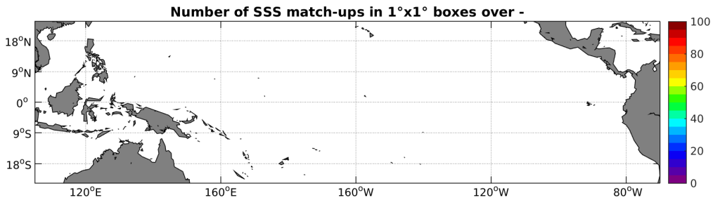
Figure 4: Number of SSS match-ups between TSG-GOSUD-Sailing-ship SSS and the AQUARIUS-L2-JPL-V4 SSS product for the Tropical Pacific Ocean Pi-MEP region over 1^\circ \times 1^\circ boxes and for the full satellite product period.
