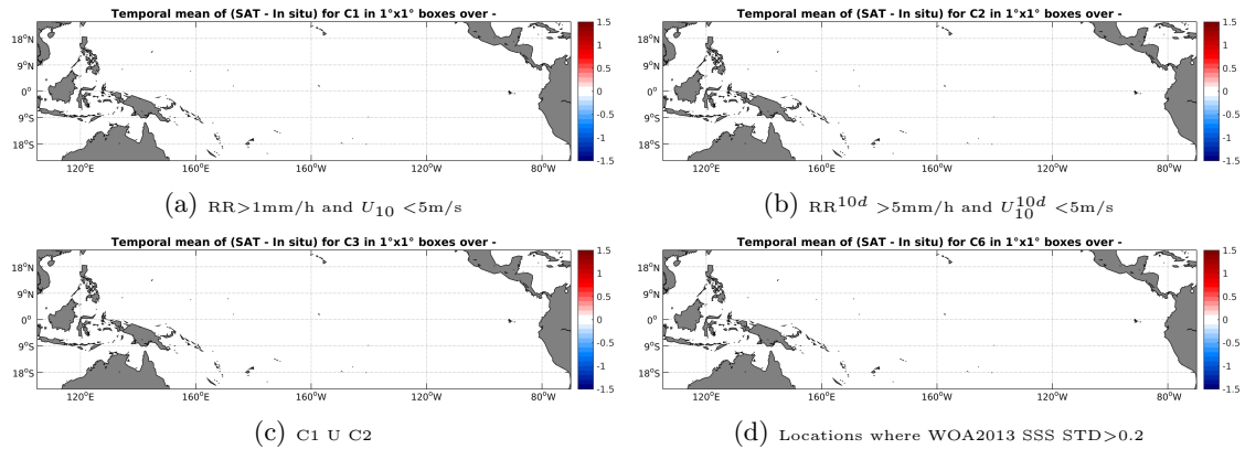
Figure 12: Temporal mean gridded over spatial boxes of size 1^\circ \times 1^\circ of \Delta SSS (AQUARIUS-L2-JPL-V4 - TSG-GOSUD-Sailing-ship) for 4 different subdatasets corresponding to:RR >1 mm/h and U_{10} < 5 m/s (a), RR^{10d} > 5 mm/h and U_{10}^{10d} < 5 m/s (b), C1 U C2 (c),Locations where WOA2013 SSS STD >0.2 (d).
