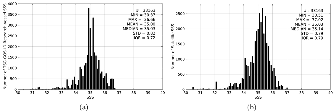
Figure 2: Histograms of SSS from TSG-GOSUD-Research-vessel (a) and AQUARIUS-L2-JPL-V4 (b) considering all match-up pairs per bins of 0.1 over the Tropical Pacific Ocean Pi-MEP region and for the full satellite product period.
