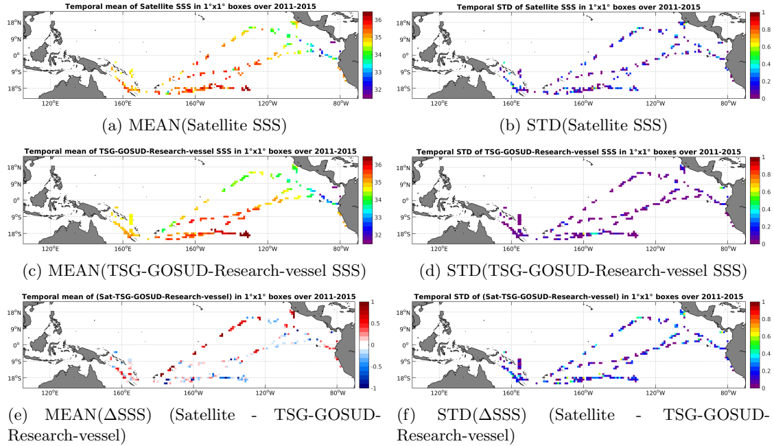
Figure 6: Temporal mean (left) and STD (right) of SSS from AQUARIUS-L2-JPL-V4 (top), TSG-GOSUD-Research-vessel (middle), and of \Delta SSS (Satellite - TSG-GOSUD-Research-vessel). Only match-up pairs are used to generate these maps.
