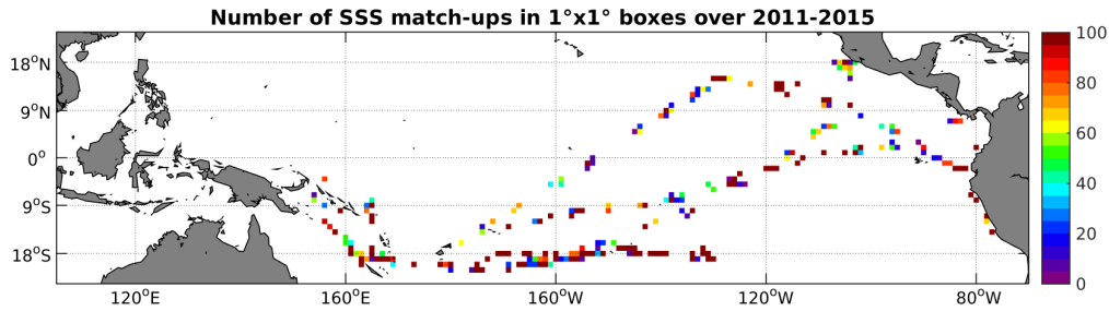
Figure 4: Number of SSS match-ups between TSG-GOSUD-Research-vessel SSS and the AQUARIUS-L2-JPL-V4 SSS product for the Tropical Pacific Ocean Pi-MEP region over 1^\circ \times 1^\circ boxes and for the full satellite product period.
