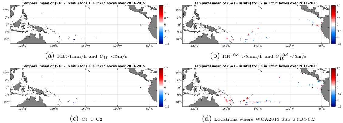
Figure 12: Temporal mean gridded over spatial boxes of size 1^\circ \times 1^\circ of \Delta SSS (AQUARIUS-L2-JPL-V4 - TSG-GOSUD-Research-vessel) for 4 different subdatasets corresponding to: RR > 1\text{mm/h} and U_{10} < 5\text{m/s} (a), RR^{10d} > 5\text{mm/h} and U_{10}^{10d} < 5\text{m/s} (b), C1 U C2 (c), Locations where WOA2013 SSS STD > 0.2 (d).
