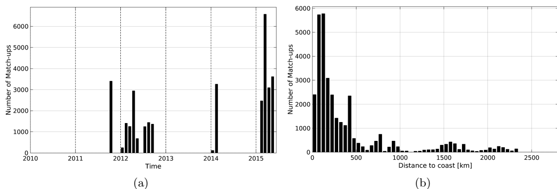
Figure 1: Number of match-ups between TSG-GOSUD-Research-vessel and AQUARIUS-L2-JPL-V4 SSS as a function of time (a) and as function of the distance to coast (b) over the Tropical Pacific Ocean Pi-MEP region and for the full satellite product period.
