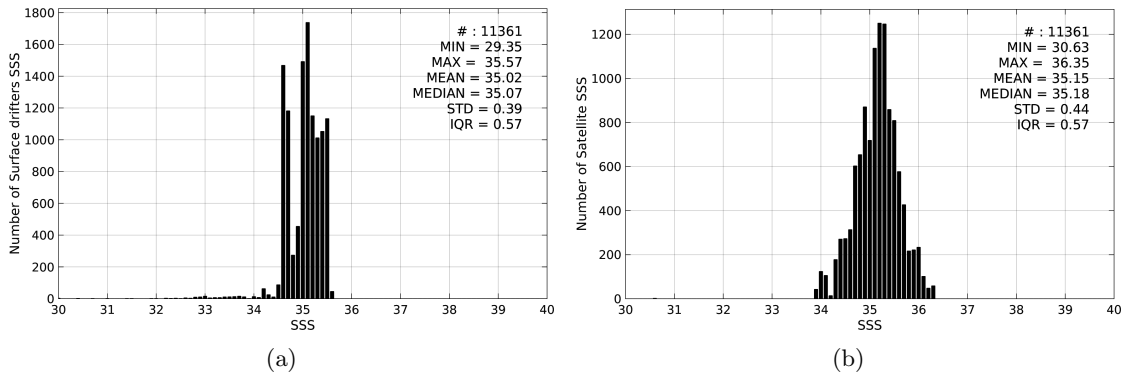
Figure 2: Histograms of SSS from Surface drifters (a) and AQUARIUS-L2-JPL-V4 (b) considering all match-up pairs per bins of 0.1 over the Tropical Pacific Ocean Pi-MEP region and for the full satellite product period.
