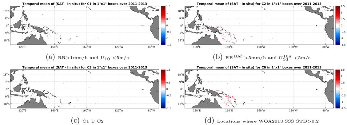
Figure 11: Temporal mean gridded over spatial boxes of size 1^\circ \times 1^\circ of \Delta SSS (AQUARIUS-L2-JPL-V4 - Surface drifters) for 4 different subdatasets corresponding to: RR > 1\text{mm/h} and U_{10} < 5\text{m/s} (a), RR^{10d} > 5\text{mm/h} and U_{10}^{10d} < 5\text{m/s} (b), C1 U C2 (c), Locations where WOA2013 SSS STD > 0.2 (d).
