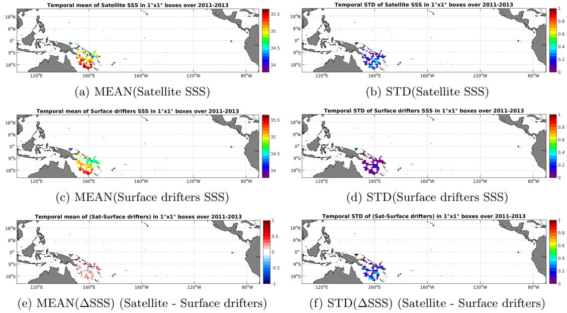
Figure 5: Temporal mean (left) and STD (right) of SSS from AQUARIUS-L2-JPL-V4 (top), Surface drifters (middle), and of \Delta SSS (Satellite - Surface drifters). Only match-up pairs are used to generate these maps.
