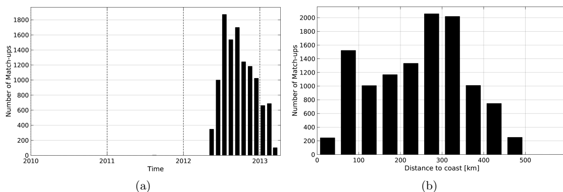
Figure 1: Number of match-ups between Surface drifters and AQUARIUS-L2-JPL-V4 SSS as a function of time (a) and as function of the distance to coast (b) over the Tropical Pacific Ocean Pi-MEP region and for the full satellite product period.
