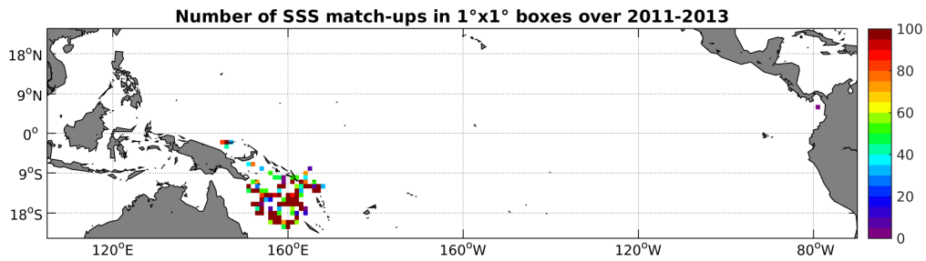
Figure 3: Number of SSS match-ups between Surface drifters SSS and the AQUARIUS-L2-JPL-V4 SSS product for the Tropical Pacific Ocean Pi-MEP region over 1°x1° boxes and for the full satellite product period.
