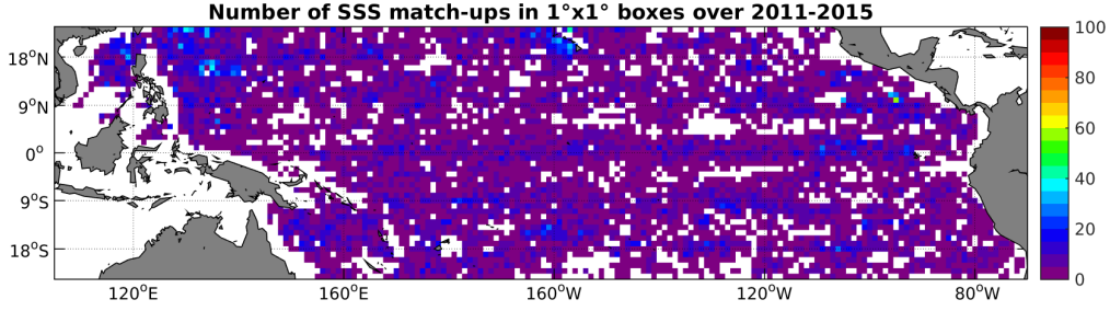
Figure 4: Number of SSS match-ups between Argo SSS and the AQUARIUS-L2-JPL-V4 SSS product for the Tropical Pacific Ocean Pi-MEP region over 1^\circ \times 1^\circ boxes and for the full satellite product period.
