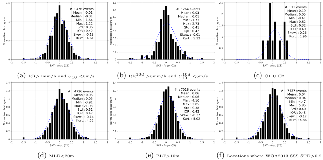
Figure 13: Normalized histogram of \Delta\text{SSS} (AQUARIUS-L2-JPL-V4 - Argo) for 6 different subdatasets corresponding to: RR > 1\text{mm/h} and U_{10} < 5\text{m/s} (a), \text{RR}^{10d} > 5\text{mm/h} and U_{10}^{10d} < 5\text{m/s} (b), C1 U C2 (c), MLD < 20\text{m} (d), BLT > 10\text{m} (e), Locations where WOA2013 SSS STD > 0.2 (f).
