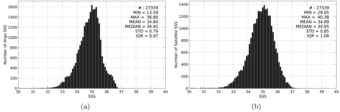
Figure 2: Histograms of SSS from Argo (a) and AQUARIUS-L2-JPL-V4 (b) considering all match-up pairs per bins of 0.1 over the Tropical Pacific Ocean Pi-MEP region and for the full satellite product period.
