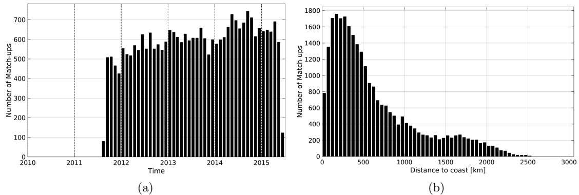
Figure 1: Number of match-ups between Argo and AQUARIUS-L2-JPL-V4 SSS as a function of time (a) and as function of the distance to coast (b) over the Tropical Pacific Ocean Pi-MEP region and for the full satellite product period.
