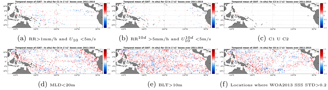
Figure 12: Temporal mean gridded over spatial boxes of size 1^\circ \times 1^\circ of \Delta\text{SSS} (AQUARIUS-L2-JPL-V4 - Argo) for 6 different subdatasets corresponding to: RR > 1\text{mm/h} and U_{10} < 5\text{m/s} (a), \text{RR}^{10d} > 5\text{mm/h} and U_{10}^{10d} < 5\text{m/s} (b), C1 U C2 (c), MLD < 20\text{m} (d), BLT > 10\text{m} (e), Locations where WOA2013 SSS STD > 0.2 (f).
