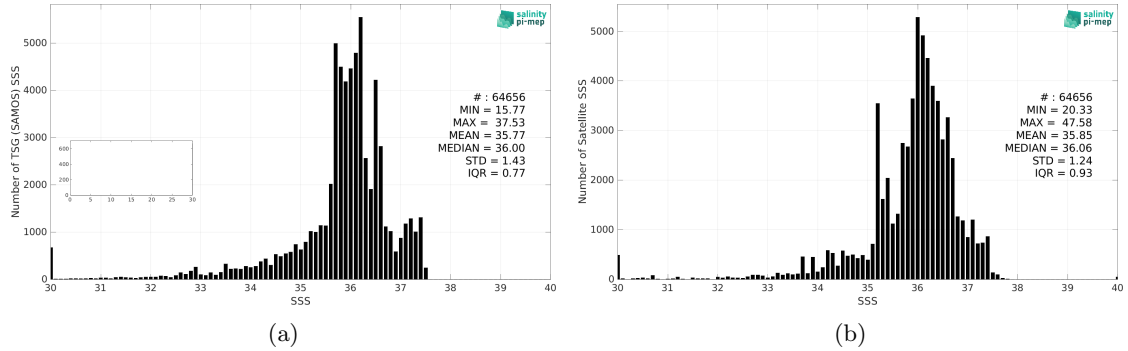
Figure 2: Histograms of SSS from TSG (SAMOS) (a) and SMOS and SMAP SSS L4 OI v1 - 7 Days (LOPS) (b) considering all match-up pairs per bins of 0.1 over the Tropical Atlantic Ocean Pi-MEP region and for the full satellite product period.
