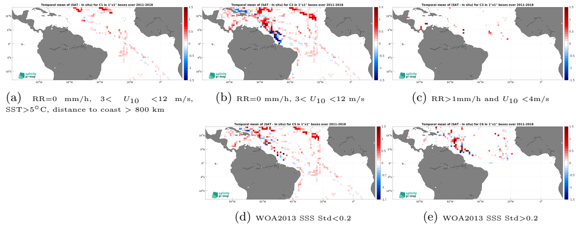
Figure 12: Temporal mean gridded over spatial boxes of size 1^\circ \times 1^\circ of \Delta\text{SSS} (SMOS and SMAP SSS L4 OI v1 - 7 Days (LOPS) - TSG (SAMOS)) for 5 different subdatasets corresponding to:RR=0 mm/h, 3 < U_{10} < 12 m/s, SST >5^\circ\text{C} , distance to coast > 800 km (a), RR=0 mm/h, 3 < U_{10} < 12 m/s (b), RR >1 mm/h and U_{10} < 4 m/s (c), WOA2013 SSS Std <0.2 (d), WOA2013 SSS Std >0.2 (e).
