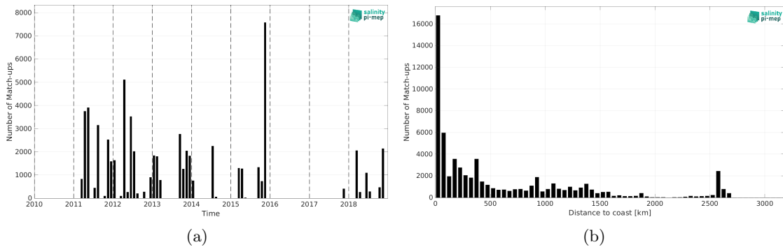
Figure 1: Number of match-ups between TSG (SAMOS) and SMOS and SMAP SSS L4 OI v1 - 7 Days (LOPS) SSS as a function of time (a) and as function of the distance to coast (b) over the Tropical Atlantic Ocean Pi-MEP region and for the full satellite product period.
