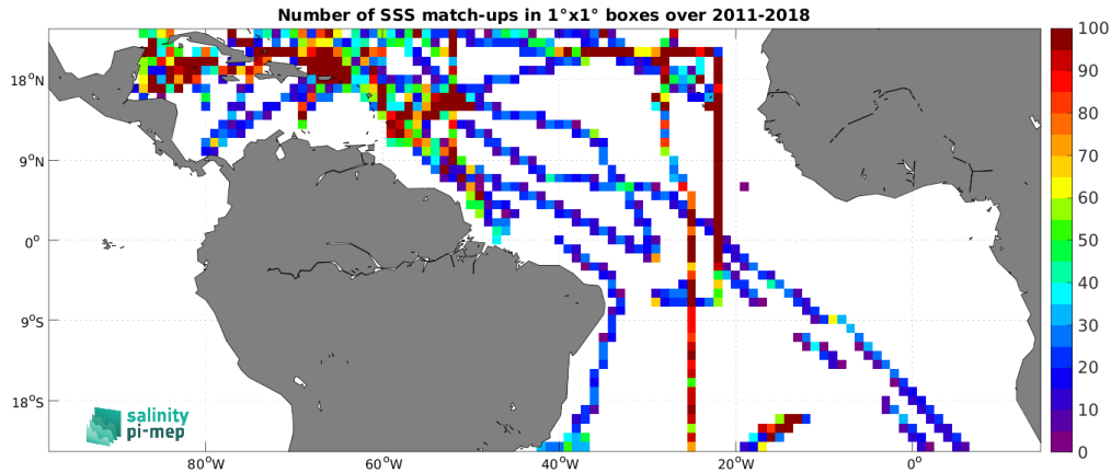
Figure 4: Number of SSS match-ups between TSG (SAMOS) SSS and the SMOS and SMAP SSS L4 OI v1 - 7 Days (LOPS) SSS product for the Tropical Atlantic Ocean Pi-MEP region over 1^\circ \times 1^\circ boxes and for the full satellite product period.
