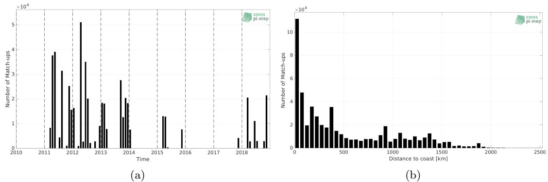
Figure 1: Number of match-ups between TSG (SAMOS) and SMOS and SMAP SSS L4 OI v1 - 7 Days (LOPS) SSS as a function of time (a) and as function of the distance to coast (b) over the Tropical Atlantic Ocean Pi-MEP region and for the full satellite product period.
