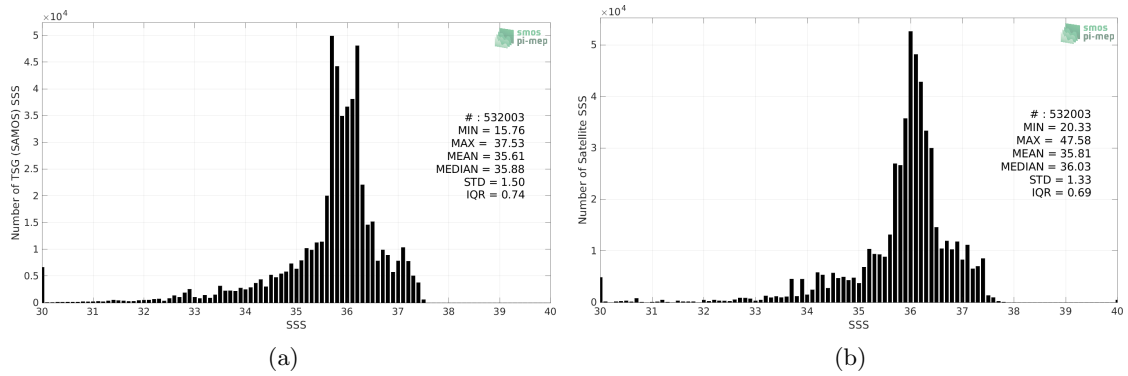
Figure 2: Histograms of SSS from TSG (SAMOS) (a) and SMOS and SMAP SSS L4 OI v1 - 7 Days (LOPS) (b) considering all match-up pairs per bins of 0.1 over the Tropical Atlantic Ocean Pi-MEP region and for the full satellite product period.
