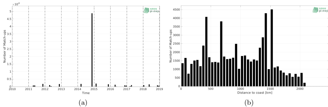
Figure 1: Number of match-ups between TSG (Polarstern) and SMOS and SMAP SSS L4 OI v1 - 7 Days (LOPS) SSS as a function of time (a) and as function of the distance to coast (b) over the Tropical Atlantic Ocean Pi-MEP region and for the full satellite product period.
