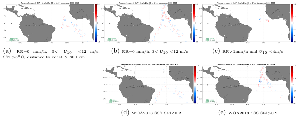
Figure 12: Temporal mean gridded over spatial boxes of size 1^\circ \times 1^\circ of \Delta\text{SSS} (SMOS and SMAP SSS L4 OI v1 - 7 Days (LOPS) - TSG (Polarstern)) for 5 different subdatasets corresponding to:RR=0 mm/h, 3 < U_{10} < 12 m/s, SST >5^\circ\text{C} , distance to coast > 800 km (a), RR=0 mm/h, 3 < U_{10} < 12 m/s (b), RR >1 mm/h and U_{10} < 4 m/s (c), WOA2013 SSS Std <0.2 (d), WOA2013 SSS Std >0.2 (e).
