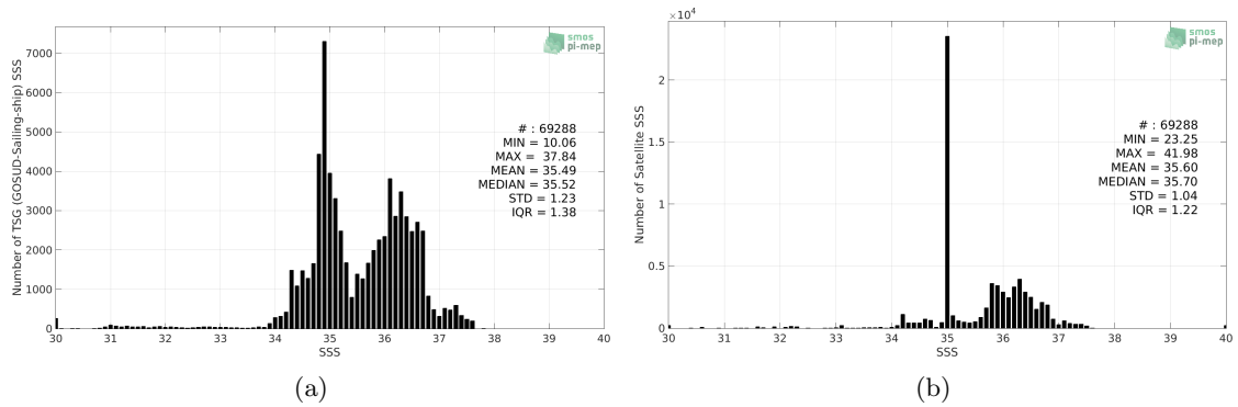
Figure 2: Histograms of SSS from TSG (GOSUD-Sailing-ship) (a) and SMOS and SMAP SSS L4 OI v1 - 7 Days (LOPS) (b) considering all match-up pairs per bins of 0.1 over the Tropical Atlantic Ocean Pi-MEP region and for the full satellite product period.
