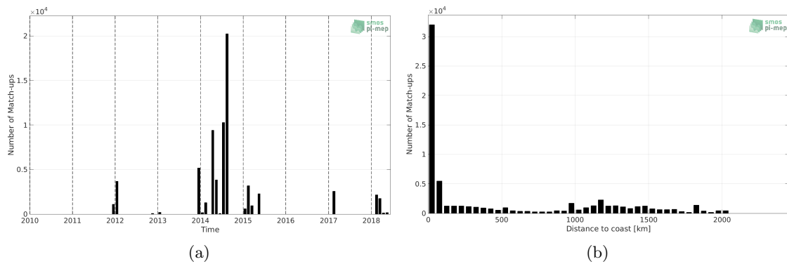
Figure 1: Number of match-ups between TSG (GOSUD-Sailing-ship) and SMOS and SMAP SSS L4 OI v1 - 7 Days (LOPS) SSS as a function of time (a) and as function of the distance to coast (b) over the Tropical Atlantic Ocean Pi-MEP region and for the full satellite product period.
