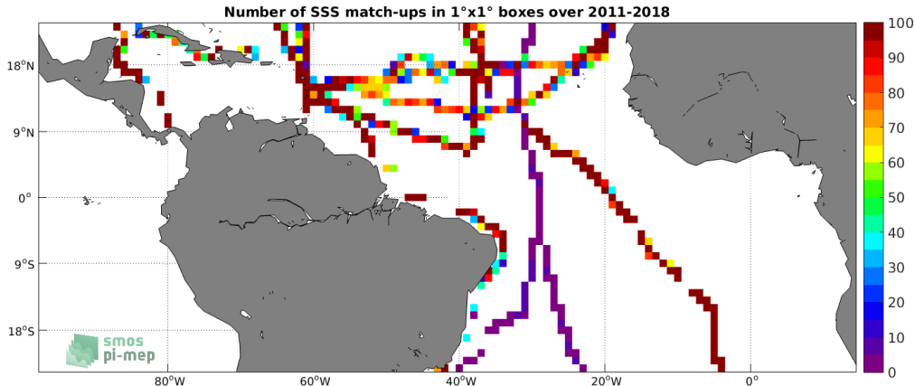
Figure 4: Number of SSS match-ups between TSG (GOSUD-Sailing-ship) SSS and the SMOS and SMAP SSS L4 OI v1 - 7 Days (LOPS) SSS product for the Tropical Atlantic Ocean Pi-MEP region over 1^\circ \times 1^\circ boxes and for the full satellite product period.
