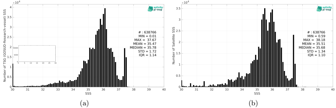
Figure 2: Histograms of SSS from TSG (GOSUD-Research-vessel) (a) and SMOS and SMAP SSS L4 OI v1 - 7 Days (LOPS) (b) considering all match-up pairs per bins of 0.1 over the Tropical Atlantic Ocean Pi-MEP region and for the full satellite product period.
