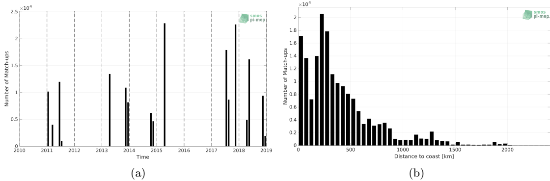
Figure 1: Number of match-ups between TSG (CSIC-UTM) and SMOS and SMAP SSS L4 OI v1 - 7 Days (LOPS) SSS as a function of time (a) and as function of the distance to coast (b) over the Tropical Atlantic Ocean Pi-MEP region and for the full satellite product period.
