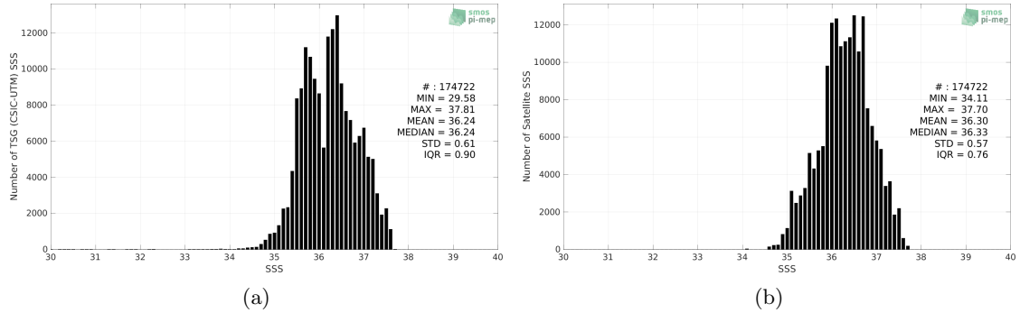
Figure 2: Histograms of SSS from TSG (CSIC-UTM) (a) and SMOS and SMAP SSS L4 OI v1 - 7 Days (LOPS) (b) considering all match-up pairs per bins of 0.1 over the Tropical Atlantic Ocean Pi-MEP region and for the full satellite product period.
