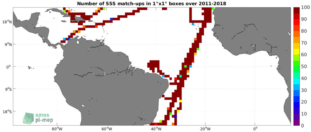
Figure 4: Number of SSS match-ups between TSG (CSIC-UTM) SSS and the SMOS and SMAP SSS L4 OI v1 - 7 Days (LOPS) SSS product for the Tropical Atlantic Ocean Pi-MEP region over 1^\circ \times 1^\circ boxes and for the full satellite product period.
