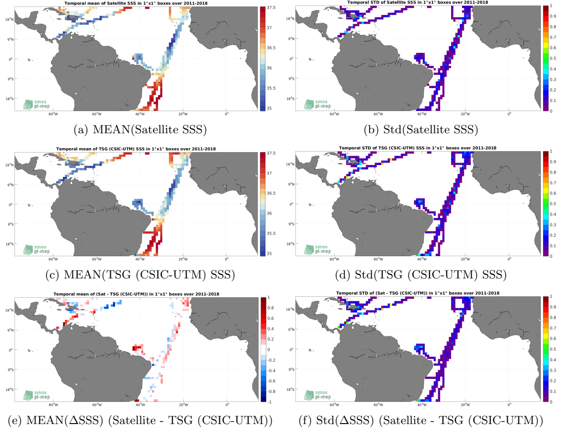
Figure 6: Temporal mean (left) and Std (right) of SSS from SMOS and SMAP SSS L4 OI v1 - 7 Days (LOPS) (top), TSG (CSIC-UTM) (middle), and of \Delta\text{SSS} (Satellite - TSG (CSIC-UTM)). Only match-up pairs are used to generate these maps.
