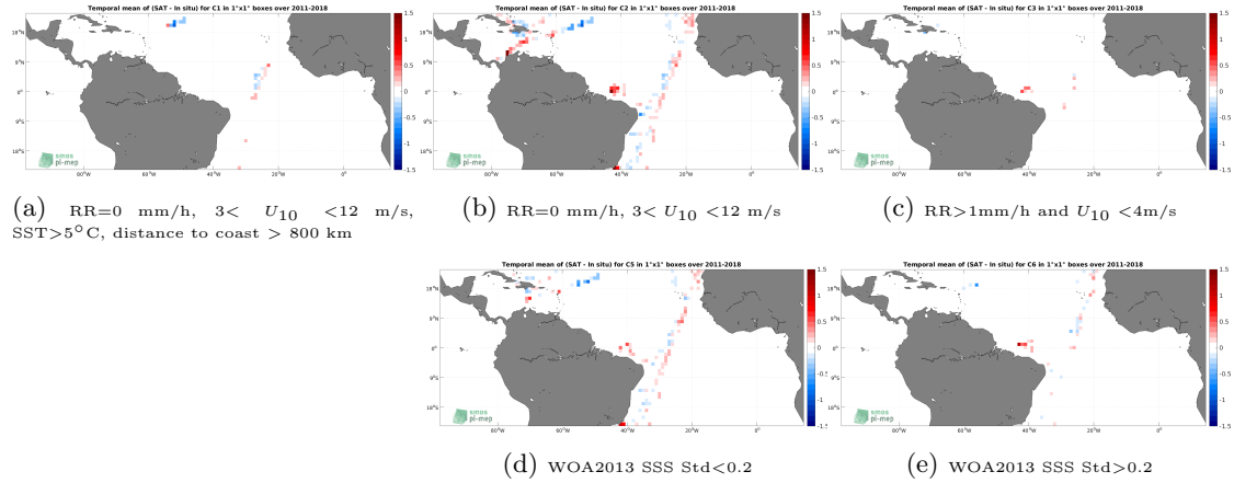
Figure 12: Temporal mean gridded over spatial boxes of size 1^{\circ}\times 1^{\circ} of \Delta\text{SSS} (SMOS and SMAP SSS L4 OI v1 - 7 Days (LOPS) - TSG (CSIC-UTM)) for 5 different subdatasets corresponding to:RR=0 mm/h, 3 < U_{10} < 12 m/s, SST > 5^{\circ}\text{C} , distance to coast > 800 km (a), RR=0 mm/h, 3 < U_{10} < 12 m/s (b), RR > 1 mm/h and U_{10} < 4 m/s (c), WOA2013 SSS Std < 0.2 (d), WOA2013 SSS Std > 0.2 (e).
