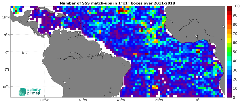
Figure 4: Number of SSS match-ups between Argo SSS and the SMOS and SMAP SSS L4 OI v1 - 7 Days (LOPS) SSS product for the Tropical Atlantic Ocean Pi-MEP region over 1^{\circ} \times 1^{\circ} boxes and for the full satellite product period.
