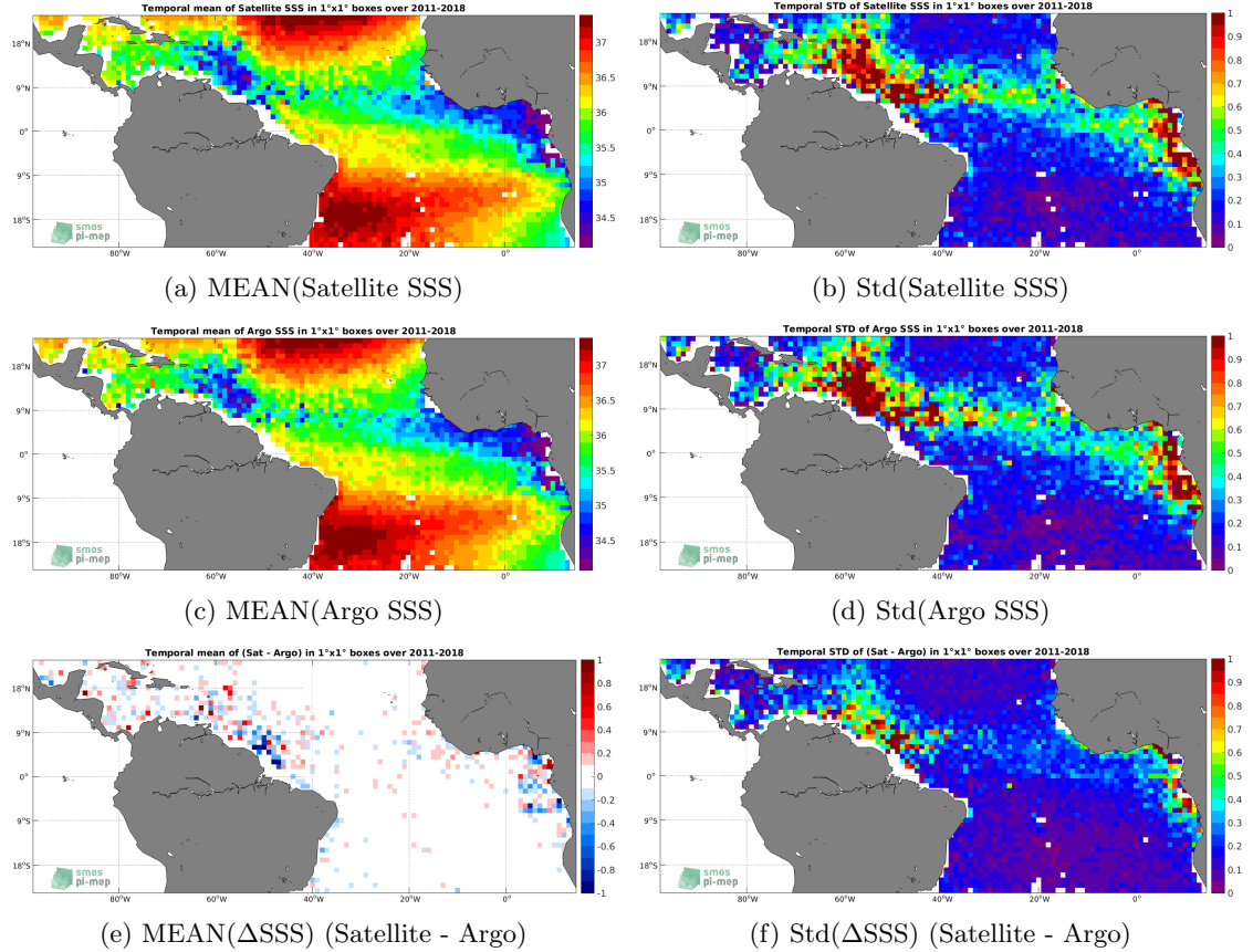
Figure 6: Temporal mean (left) and Std (right) of SSS from SMOS and SMAP SSS L4 OI v1 - 7 Days (LOPS) (top), Argo (middle), and of \Delta\text{SSS} (Satellite - Argo). Only match-up pairs are used to generate these maps.
