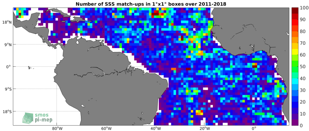
Figure 4: Number of SSS match-ups between Argo SSS and the SMOS and SMAP SSS L4 OI v1 - 7 Days (LOPS) SSS product for the Tropical Atlantic Ocean Pi-MEP region over 1^\circ \times 1^\circ boxes and for the full satellite product period.
