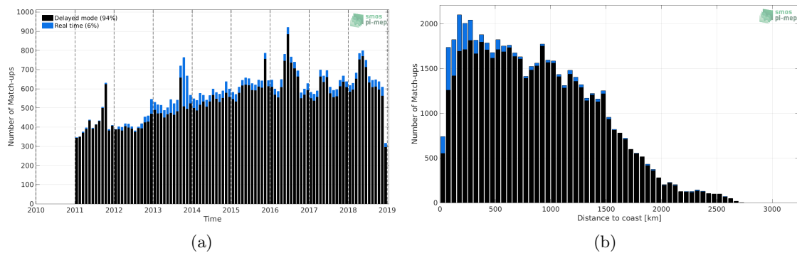
Figure 1: Number of match-ups between Argo and SMOS and SMAP SSS L4 OI v1 - 7 Days (LOPS) SSS as a function of time (a) and as function of the distance to coast (b) over the Tropical Atlantic Ocean Pi-MEP region and for the full satellite product period.
