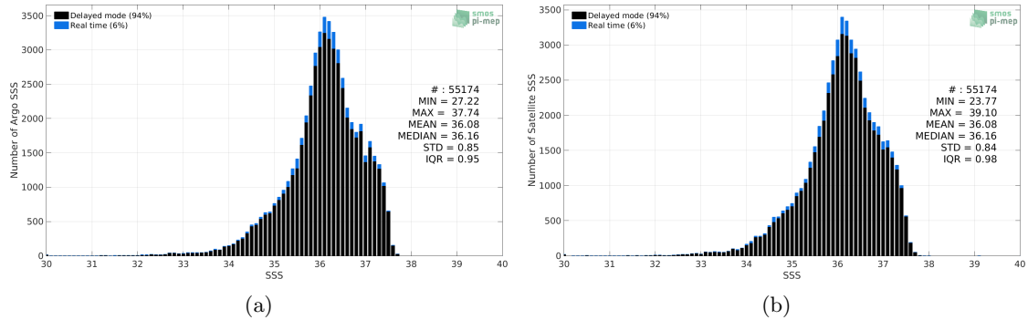
Figure 2: Histograms of SSS from Argo (a) and SMOS and SMAP SSS L4 OI v1 - 7 Days (LOPS) (b) considering all match-up pairs per bins of 0.1 over the Tropical Atlantic Ocean Pi-MEP region and for the full satellite product period.
