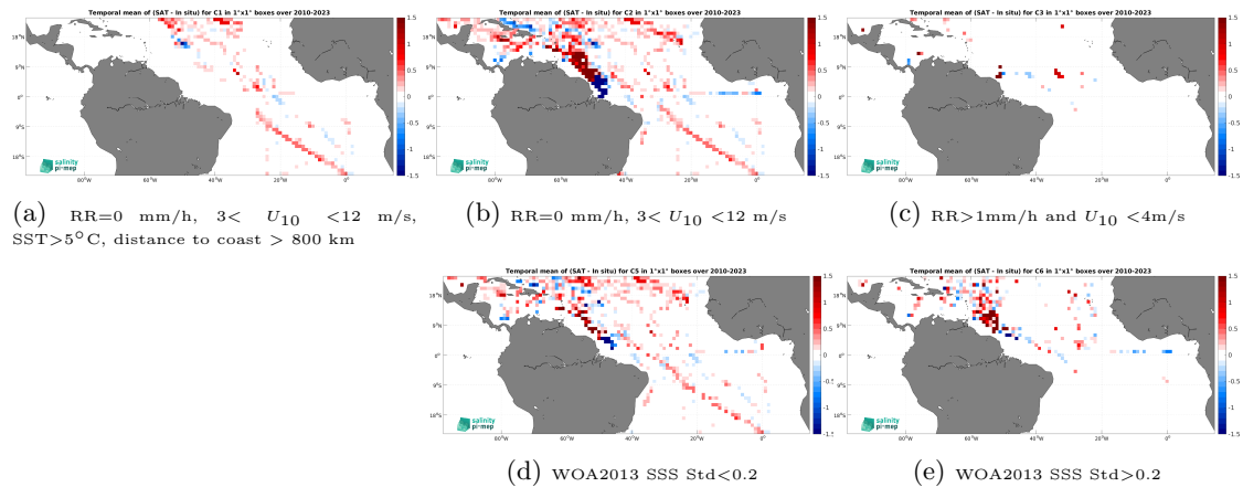
Figure 12: Temporal mean gridded over spatial boxes of size 1^\circ \times 1^\circ of \Delta\text{SSS} (SMOS SSS L4 v1 - Weekly (CMEMS-CNR) - TSG (SAMOS)) for 5 different subdatasets corresponding to:RR=0 mm/h, 3 < U_{10} < 12 m/s, SST >5^\circ\text{C} , distance to coast > 800 km (a), RR=0 mm/h, 3 < U_{10} < 12 m/s (b), RR >1 mm/h and U_{10} < 4 m/s (c), WOA2013 SSS Std <0.2 (d), WOA2013 SSS Std >0.2 (e).
