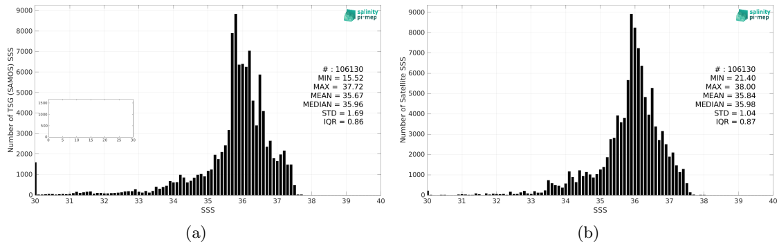
Figure 2: Histograms of SSS from TSG (SAMOS) (a) and SMOS SSS L4 v1 - Weekly (CMEMS-CNR) (b) considering all match-up pairs per bins of 0.1 over the Tropical Atlantic Ocean Pi-MEP region and for the full satellite product period.
