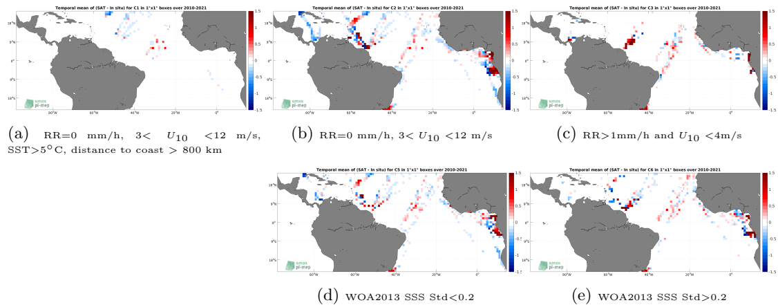
Figure 12: Temporal mean gridded over spatial boxes of size 1^\circ \times 1^\circ of \Delta\text{SSS} (SMOS SSS L4 v1 - Weekly (CMEMS-CNR) - TSG (LEGOS-DM)) for 5 different subdatasets corresponding to:RR=0 mm/h, 3 < U_{10} < 12 m/s, SST >5^\circ\text{C} , distance to coast > 800 km (a), RR=0 mm/h, 3 < U_{10} < 12 m/s (b), RR >1 mm/h and U_{10} < 4 m/s (c), WOA2013 SSS Std <0.2 (d), WOA2013 SSS Std >0.2 (e).
