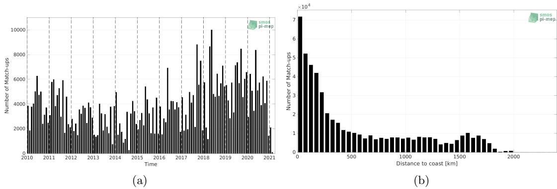
Figure 1: Number of match-ups between TSG (LEGOS-DM) and SMOS SSS L4 v1 - Weekly (CMEMS-CNR) SSS as a function of time (a) and as function of the distance to coast (b) over the Tropical Atlantic Ocean Pi-MEP region and for the full satellite product period.
