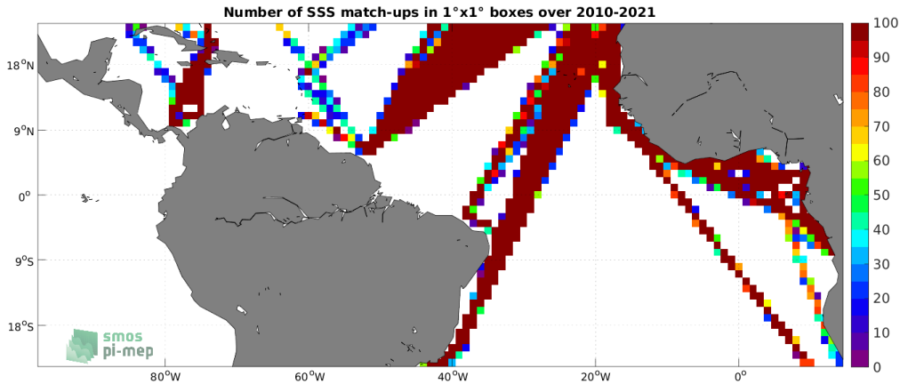
Figure 4: Number of SSS match-ups between TSG (LEGOS-DM) SSS and the SMOS SSS L4 v1 - Weekly (CMEMS-CNR) SSS product for the Tropical Atlantic Ocean Pi-MEP region over 1^\circ \times 1^\circ boxes and for the full satellite product period.
