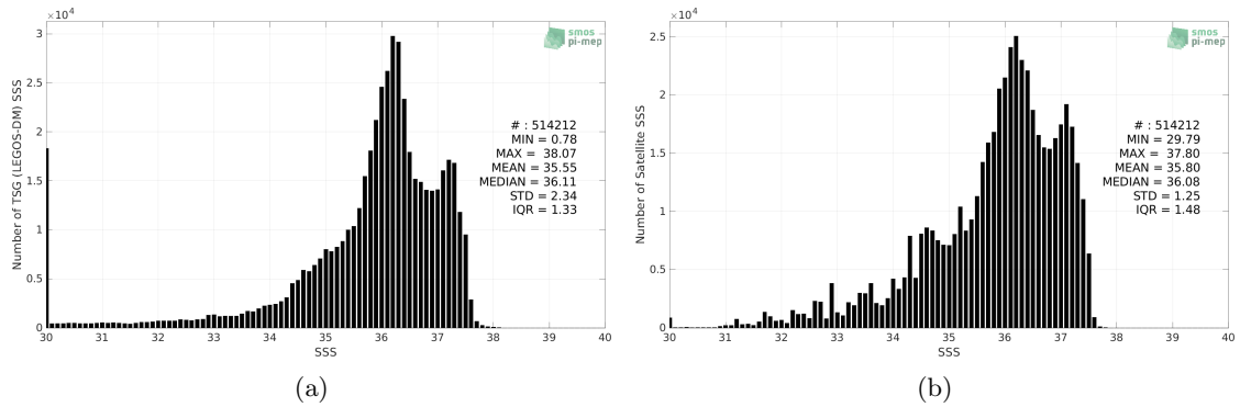
Figure 2: Histograms of SSS from TSG (LEGOS-DM) (a) and SMOS SSS L4 v1 - Weekly (CMEMS-CNR) (b) considering all match-up pairs per bins of 0.1 over the Tropical Atlantic Ocean Pi-MEP region and for the full satellite product period.
