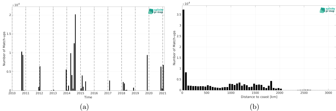
Figure 1: Number of match-ups between TSG (GOSUD-Sailing-ship) and SMOS SSS L4 v1 - Weekly (CMEMS-CNR) SSS as a function of time (a) and as function of the distance to coast (b) over the Tropical Atlantic Ocean Pi-MEP region and for the full satellite product period.
