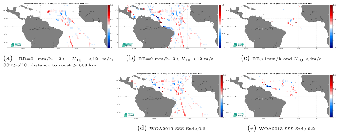
Figure 12: Temporal mean gridded over spatial boxes of size 1^\circ \times 1^\circ of \Delta\text{SSS} (SMOS SSS L4 v1 - Weekly (CMEMS-CNR) - TSG (GOSUD-Sailing-ship)) for 5 different subdatasets corresponding to:RR=0 mm/h, 3 < U_{10} < 12 m/s, SST>5°C, distance to coast > 800 km (a), RR=0 mm/h, 3 < U_{10} < 12 m/s (b), RR>1mm/h and U_{10} < 4 m/s (c), WOA2013 SSS Std<0.2 (d), WOA2013 SSS Std>0.2 (e).
