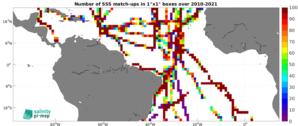
Figure 4: Number of SSS match-ups between TSG (GOSUD-Sailing-ship) SSS and the SMOS SSS L4 v1 - Weekly (CMEMS-CNR) SSS product for the Tropical Atlantic Ocean Pi-MEP region over 1^\circ \times 1^\circ boxes and for the full satellite product period.
