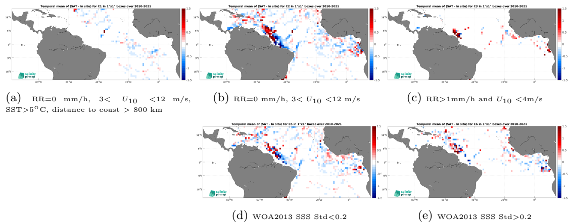
Figure 12: Temporal mean gridded over spatial boxes of size 1^\circ \times 1^\circ of \Delta\text{SSS} (SMOS SSS L4 v1 - Weekly (CMEMS-CNR) - TSG (GOSUD-Research-vessel)) for 5 different subdatasets corresponding to:RR=0 mm/h, 3 < U_{10} < 12 m/s, SST>5°C, distance to coast > 800 km (a), RR=0 mm/h, 3 < U_{10} < 12 m/s (b), RR>1mm/h and U_{10} < 4 m/s (c), WOA2013 SSS Std<0.2 (d), WOA2013 SSS Std>0.2 (e).
