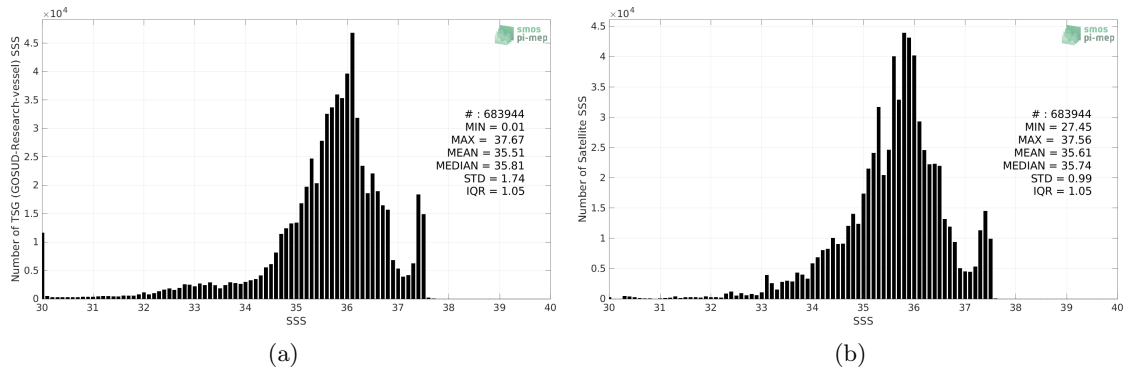
Figure 2: Histograms of SSS from TSG (GOSUD-Research-vessel) (a) and SMOS SSS L4 v1 - Weekly (CMEMS-CNR) (b) considering all match-up pairs per bins of 0.1 over the Tropical Atlantic Ocean Pi-MEP region and for the full satellite product period.
