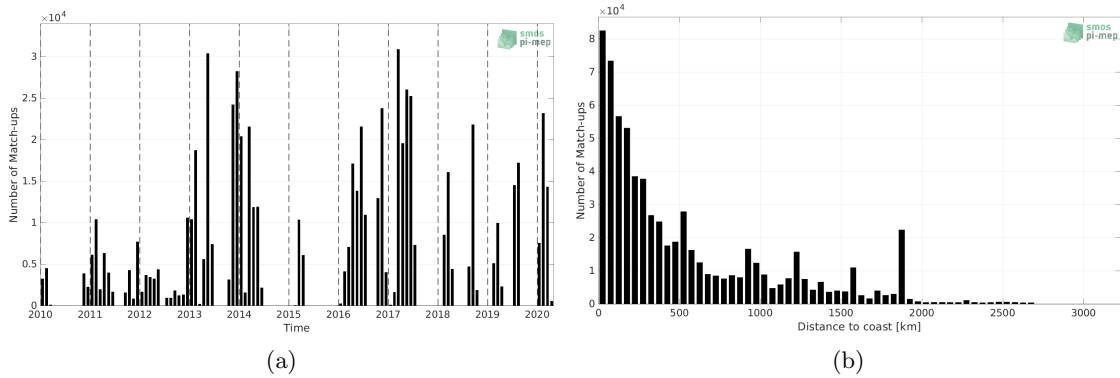
Figure 1: Number of match-ups between TSG (GOSUD-Research-vessel) and SMOS SSS L4 v1 - Weekly (CMEMS-CNR) SSS as a function of time (a) and as function of the distance to coast (b) over the Tropical Atlantic Ocean Pi-MEP region and for the full satellite product period.
