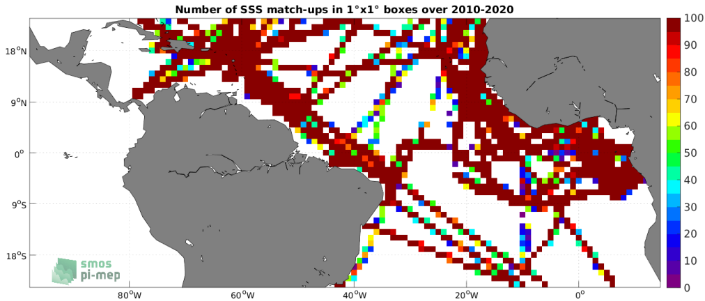
Figure 4: Number of SSS match-ups between TSG (GOSUD-Research-vessel) SSS and the SMOS SSS L4 v1 - Weekly (CMEMS-CNR) SSS product for the Tropical Atlantic Ocean Pi-MEP region over 1^\circ \times 1^\circ boxes and for the full satellite product period.
