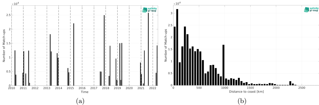
Figure 1: Number of match-ups between TSG (CSIC-UTM) and SMOS SSS L4 v1 - Weekly (CMEMS-CNR) SSS as a function of time (a) and as function of the distance to coast (b) over the Tropical Atlantic Ocean Pi-MEP region and for the full satellite product period.
