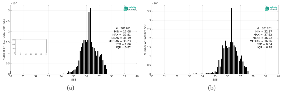
Figure 2: Histograms of SSS from TSG (CSIC-UTM) (a) and SMOS SSS L4 v1 - Weekly (CMEMS-CNR) (b) considering all match-up pairs per bins of 0.1 over the Tropical Atlantic Ocean Pi-MEP region and for the full satellite product period.
