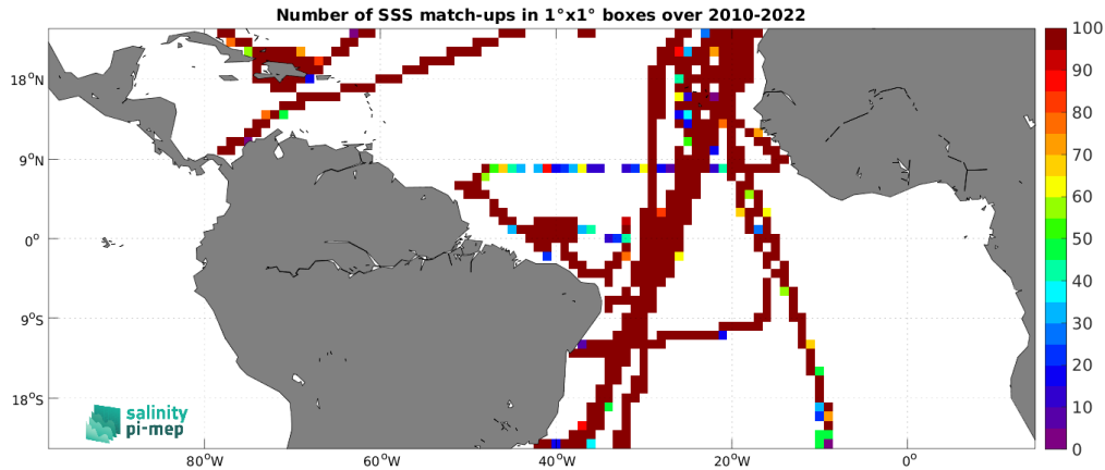
Figure 4: Number of SSS match-ups between TSG (CSIC-UTM) SSS and the SMOS SSS L4 v1 - Weekly (CMEMS-CNR) SSS product for the Tropical Atlantic Ocean Pi-MEP region over 1^\circ \times 1^\circ boxes and for the full satellite product period.
