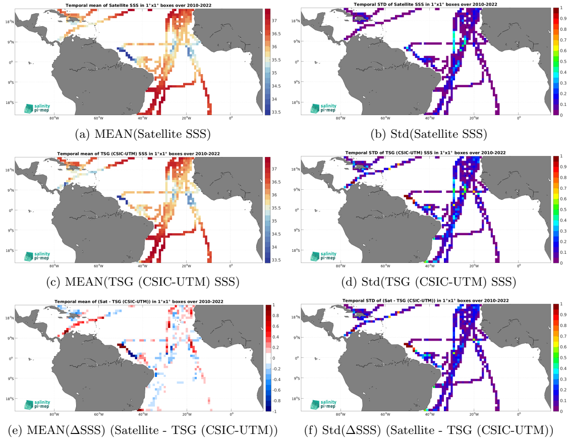
Figure 6: Temporal mean (left) and Std (right) of SSS from SMOS SSS L4 v1 - Weekly (CMEMS-CNR) (top), TSG (CSIC-UTM) (middle), and of \Delta\text{SSS}(\text{Satellite} - \text{TSG}(\text{CSIC-UTM})) . Only match-up pairs are used to generate these maps.
