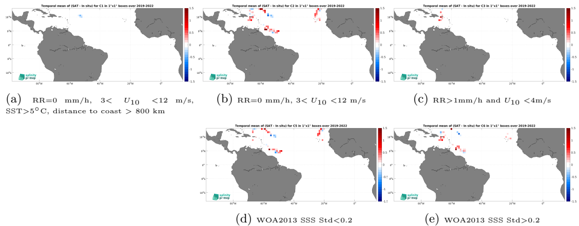
Figure 12: Temporal mean gridded over spatial boxes of size 1^\circ \times 1^\circ of \Delta\text{SSS} (SMOS SSS L4 v1 - Weekly (CMEMS-CNR) - Sailability) for 5 different subdatasets corresponding to:RR=0 mm/h, 3 < U_{10} < 12 m/s, SST >5^\circ\text{C} , distance to coast > 800 km (a), RR=0 mm/h, 3 < U_{10} < 12 m/s (b), RR >1 mm/h and U_{10} < 4 m/s (c), WOA2013 SSS Std <0.2 (d), WOA2013 SSS Std >0.2 (e).
