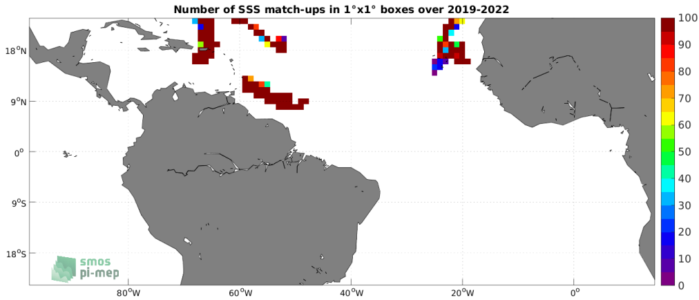
Figure 4: Number of SSS match-ups between Saildrone SSS and the SMOS SSS L4 v1 - Weekly (CMEMS-CNR) SSS product for the Tropical Atlantic Ocean Pi-MEP region over 1^\circ \times 1^\circ boxes and for the full satellite product period.
