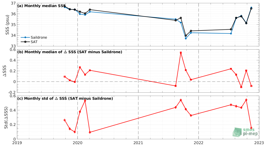
Figure 7: Time series of the monthly median SSS (top), median of \Delta SSS (Satellite - Sairdrone) and Std of \Delta SSS (Satellite - Sairdrone) over the Tropical Atlantic Ocean Pi-MEP region considering all match-ups collected by the Pi-MEP.
