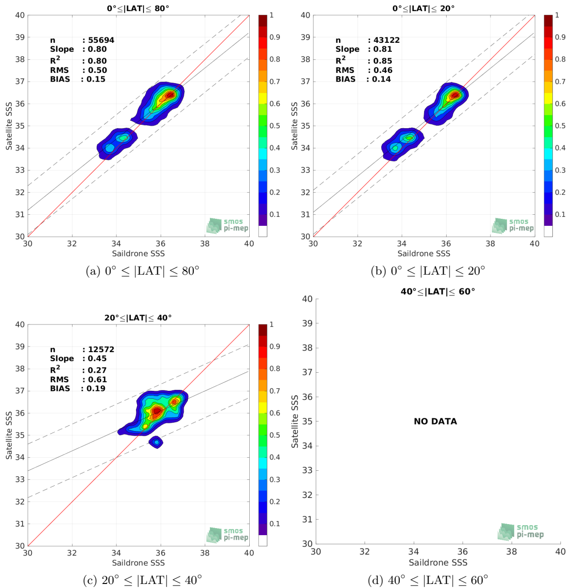
Figure 9: Contour maps of the concentration of SMOS SSS L4 v1 - Weekly (CMEMS-CNR) SSS (y-axis) versus Saïldrone SSS (x-axis) at match-up pairs for different latitude bands. For each plot, the red line shows x=y . The black thin and dashed lines indicate a linear fit through the data cloud and the \pm 95\% confidence levels, respectively. The number match-up pairs n , the slope and R^2 coefficient of the linear fit, the root mean square (RMS) and the mean bias between satellite and in situ data are indicated for each latitude band in each plots.
