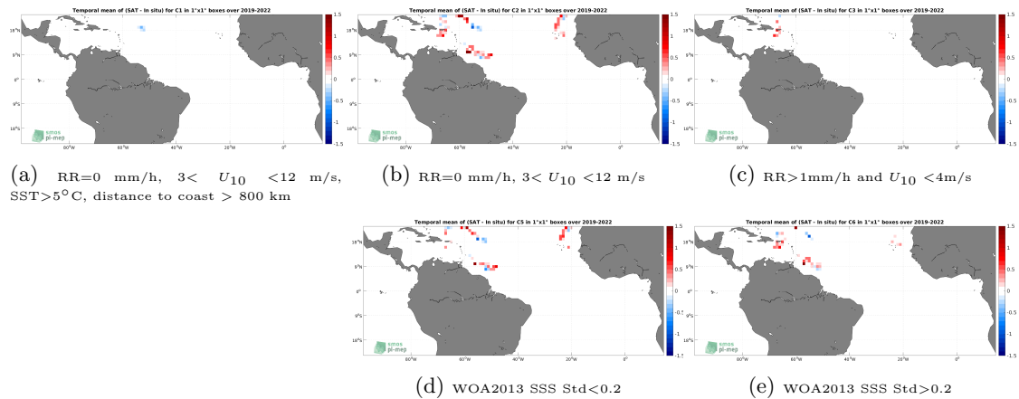
Figure 12: Temporal mean gridded over spatial boxes of size 1^\circ \times 1^\circ of \Delta\text{SSS} (SMOS SSS L4 v1 - Weekly (CMEMS-CNR) - Saildrone) for 5 different subdatasets corresponding to:RR=0 mm/h, 3 < U_{10} < 12 m/s, SST >5^\circ\text{C} , distance to coast > 800 km (a), RR=0 mm/h, 3 < U_{10} < 12 m/s (b), RR >1 mm/h and U_{10} < 4 m/s (c), WOA2013 SSS Std <0.2 (d), WOA2013 SSS Std >0.2 (e).
