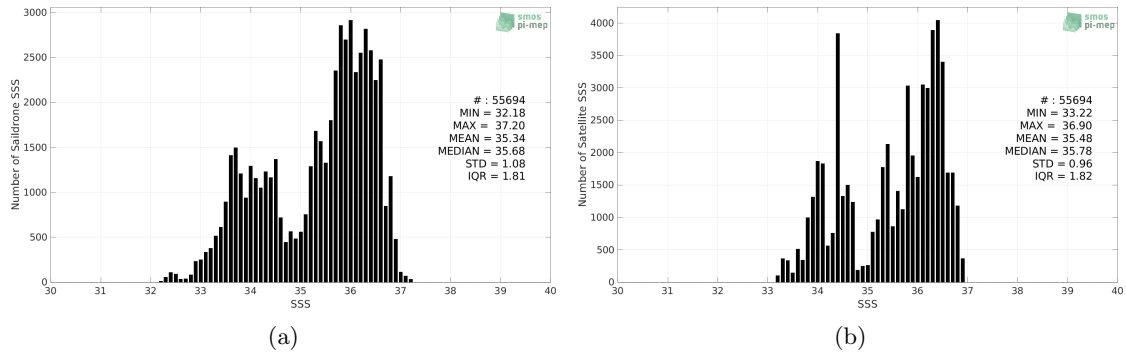
Figure 2: Histograms of SSS from Saildrone (a) and SMOS SSS L4 v1 - Weekly (CMEMS-CNR) (b) considering all match-up pairs per bins of 0.1 over the Tropical Atlantic Ocean Pi-MEP region and for the full satellite product period.
