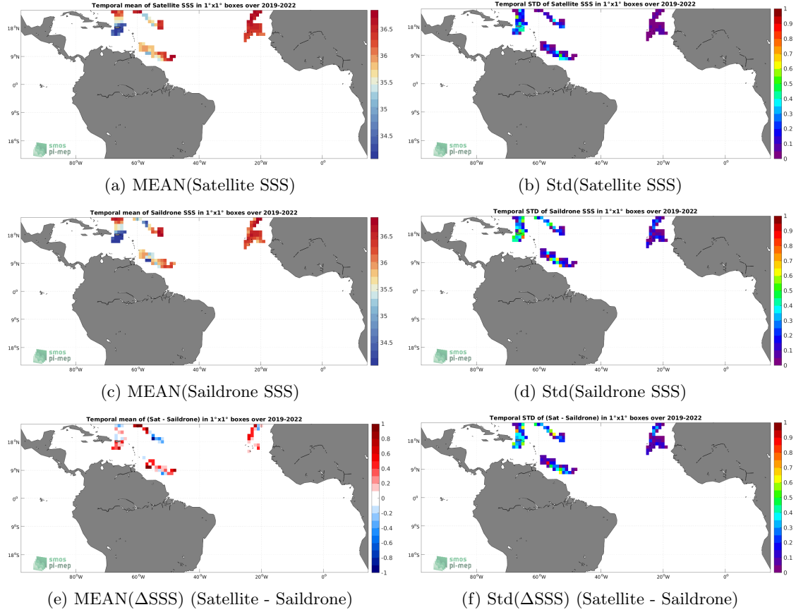
Figure 6: Temporal mean (left) and Std (right) of SSS from SMOS SSS L4 v1 - Weekly (CMEMS-CNR) (top), Saildrone (middle), and of \Delta\text{SSS} (Satellite - Saildrone). Only match-up pairs are used to generate these maps.
