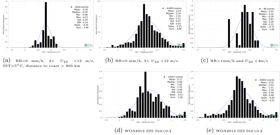
Figure 13: Normalized histogram of \Delta SSS (SMOS SSS L4 v1 - Weekly (CMEMS-CNR) - Saildrone) for 5 different subdatasets corresponding to: RR=0 mm/h, 3 < U_{10} < 12 m/s, SST > 5°C, distance to coast > 800 km (a), RR=0 mm/h, 3 < U_{10} < 12 m/s (b), RR > 1mm/h and U_{10} < 4 m/s (c), WOA2013 SSS Std < 0.2 (d), WOA2013 SSS Std > 0.2 (e).
