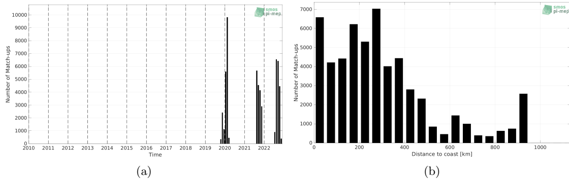
Figure 1: Number of match-ups between Saildrone and SMOS SSS L4 v1 - Weekly (CMEMS-CNR) SSS as a function of time (a) and as function of the distance to coast (b) over the Tropical Atlantic Ocean Pi-MEP region and for the full satellite product period.
