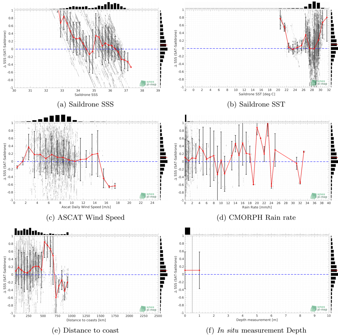
Figure 11: \Delta SSS (Satellite - Saildrone) sorted as function of SSS values a), SST b), ASCAT Wind speed c), CMORPH rain rate d), distance to coast (e) and in situ measurement depth (f). In all plots the median and Std of \Delta SSS for each bin is indicated by the red curves and black vertical thick bars ( \pm 1 Std)
