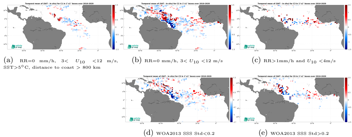
Figure 11: Temporal mean gridded over spatial boxes of size 1^\circ \times 1^\circ of \Delta\text{SSS} (SMOS SSS L4 v1 - Weekly (CMEMS-CNR) - Surface drifters) for 5 different subdatasets corresponding to:RR=0 mm/h, 3 < U_{10} < 12 m/s, SST >5^\circ\text{C} , distance to coast > 800 km (a), RR=0 mm/h, 3 < U_{10} < 12 m/s (b), RR >1 mm/h and U_{10} < 4 m/s (c), WOA2013 SSS Std <0.2 (d), WOA2013 SSS Std >0.2 (e).
