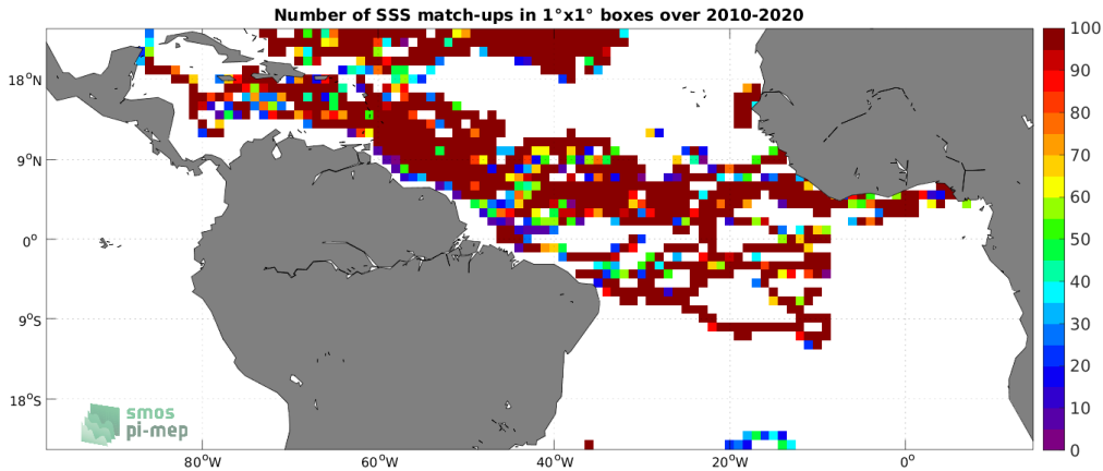
Figure 3: Number of SSS match-ups between Surface drifters SSS and the SMOS SSS L4 v1 - Weekly (CMEMS-CNR) SSS product for the Tropical Atlantic Ocean Pi-MEP region over 1^\circ \times 1^\circ boxes and for the full satellite product period.
