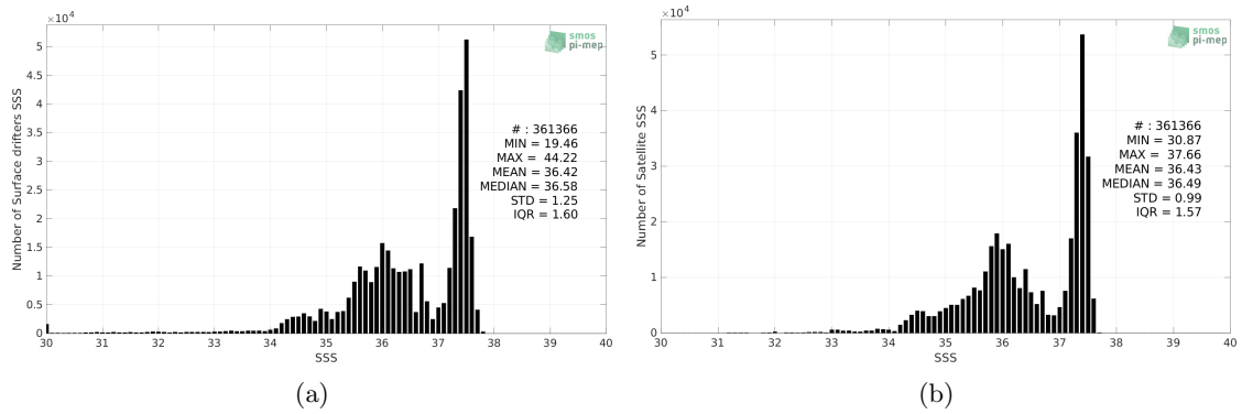
Figure 2: Histograms of SSS from Surface drifters (a) and SMOS SSS L4 v1 - Weekly (CMEMS-CNR) (b) considering all match-up pairs per bins of 0.1 over the Tropical Atlantic Ocean Pi-MEP region and for the full satellite product period.
