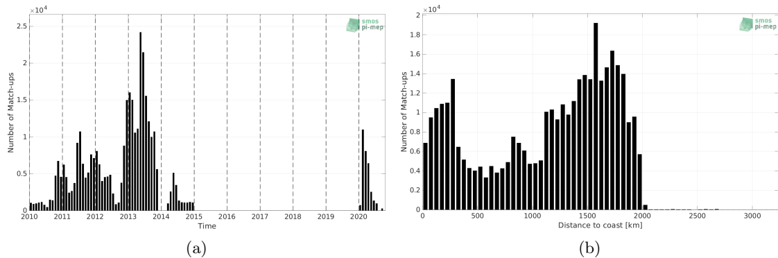
Figure 1: Number of match-ups between Surface drifters and SMOS SSS L4 v1 - Weekly (CMEMS-CNR) SSS as a function of time (a) and as function of the distance to coast (b) over the Tropical Atlantic Ocean Pi-MEP region and for the full satellite product period.
