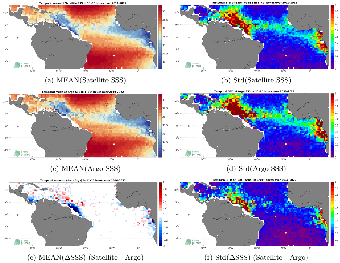
Figure 6: Temporal mean (left) and Std (right) of SSS from SMOS SSS L4 v1 - Weekly (CMEMS-CNR) (top), Argo (middle), and of \Delta SSS (Satellite - Argo). Only match-up pairs are used to generate these maps.
