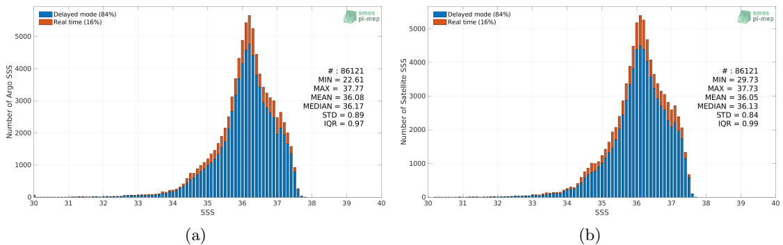
Figure 2: Histograms of SSS from Argo (a) and SMOS SSS L4 v1 - Weekly (CMEMS-CNR) (b) considering all match-up pairs per bins of 0.1 over the Tropical Atlantic Ocean Pi-MEP region and for the full satellite product period.
