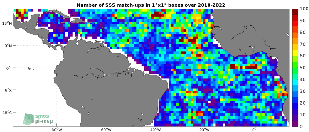
Figure 4: Number of SSS match-ups between Argo SSS and the SMOS SSS L4 v1 - Weekly (CMEMS-CNR) SSS product for the Tropical Atlantic Ocean Pi-MEP region over 1^\circ \times 1^\circ boxes and for the full satellite product period.
