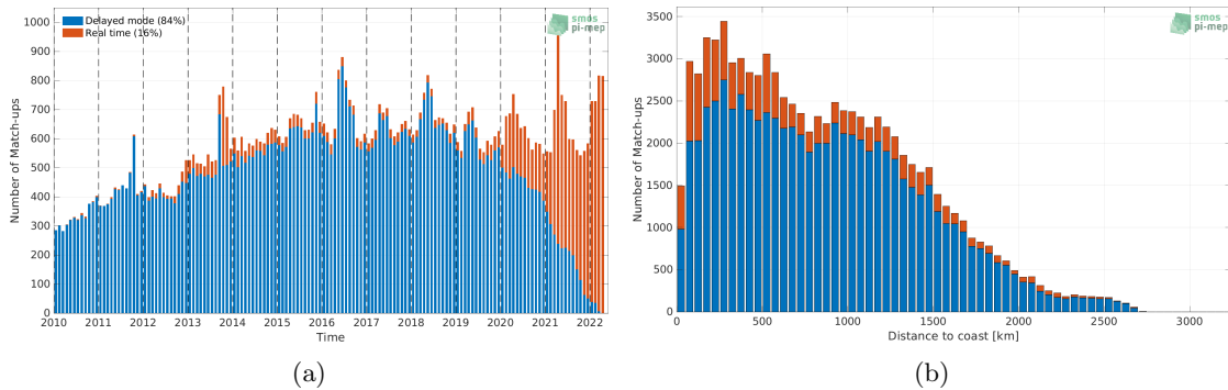
Figure 1: Number of match-ups between Argo and SMOS SSS L4 v1 - Weekly (CMEMS-CNR) SSS as a function of time (a) and as function of the distance to coast (b) over the Tropical Atlantic Ocean Pi-MEP region and for the full satellite product period.
