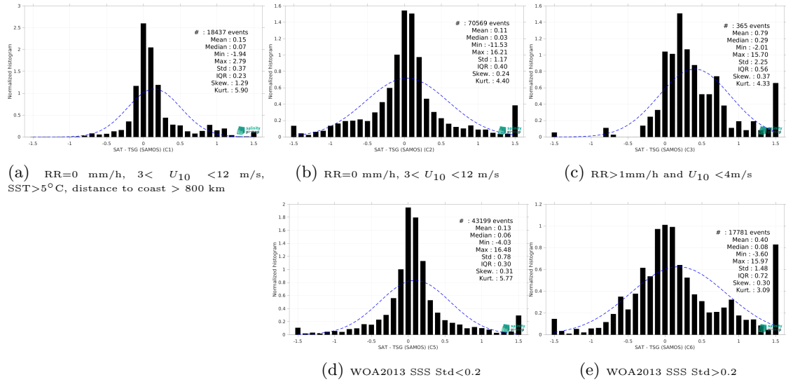
Figure 15: Normalized histogram of \Delta\text{SSS} (SMOS SSS L4 v1 - Monthly (CMEMS-CNR) - TSG (SAMOS)) for 5 different subdatasets corresponding to: RR=0 mm/h, 3 < U_{10} < 12 m/s, SST > 5^\circ\text{C} , distance to coast > 800 km (a), RR=0 mm/h, 3 < U_{10} < 12 m/s (b), RR > 1 mm/h and U_{10} < 4 m/s (c), WOA2013 SSS Std < 0.2 (d), WOA2013 SSS Std > 0.2 (e).
