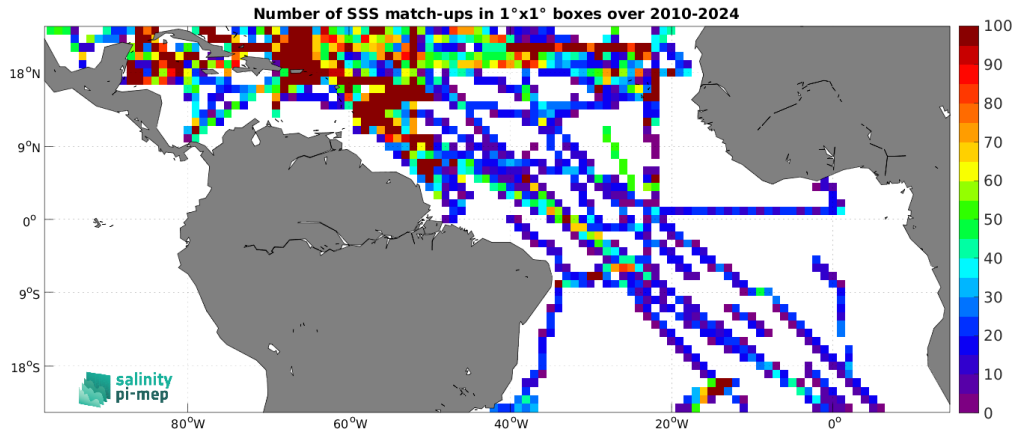
Figure 5: Number of SSS match-ups between TSG (SAMOS) SSS and the SMOS SSS L4 v1 - Monthly (CMEMS-CNR) SSS product for the Tropical Atlantic Ocean Pi-MEP region over 1^\circ \times 1^\circ boxes and for the full satellite product period.
