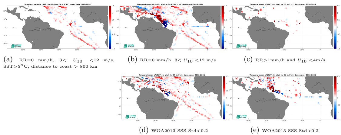
Figure 14: Temporal mean gridded over spatial boxes of size 1^\circ \times 1^\circ of \Delta\text{SSS} (SMOS SSS L4 v1 - Monthly (CMEMS-CNR) - TSG (SAMOS)) for 5 different subdatasets corresponding to:RR=0 mm/h, 3 < U_{10} < 12 m/s, SST >5^\circ\text{C} , distance to coast > 800 km (a), RR=0 mm/h, 3 < U_{10} < 12 m/s (b), RR >1 mm/h and U_{10} < 4 m/s (c), WOA2013 SSS Std <0.2 (d), WOA2013 SSS Std >0.2 (e).
