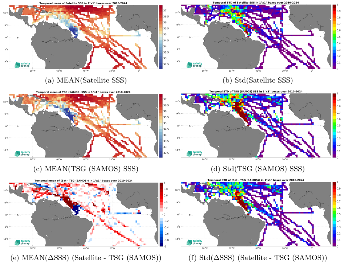
Figure 7: Temporal mean (left) and Std (right) of SSS from SMOS SSS L4 v1 - Monthly (CMEMS-CNR) (top), TSG (SAMOS) (middle), and of \Delta\text{SSS} (Satellite - TSG (SAMOS)). Only match-up pairs are used to generate these maps.
