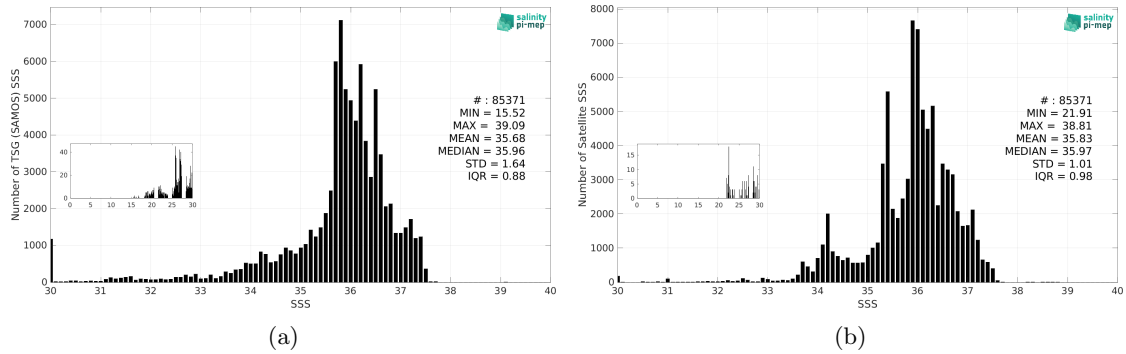
Figure 3: Histograms of SSS from TSG (SAMOS) (a) and SMOS SSS L4 v1 - Monthly (CMEMS-CNR) (b) considering all match-up pairs per bins of 0.1 over the Tropical Atlantic Ocean Pi-MEP region and for the full satellite product period.
