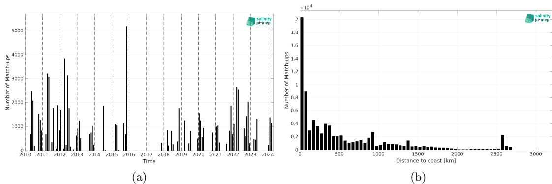
Figure 2: Number of match-ups between TSG (SAMOS) and SMOS SSS L4 v1 - Monthly (CMEMS-CNR) SSS as a function of time (a) and as function of the distance to coast (b) over the Tropical Atlantic Ocean Pi-MEP region and for the full satellite product period.
