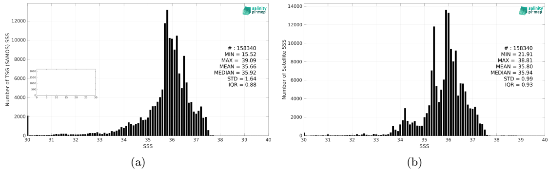
Figure 2: Histograms of SSS from TSG (SAMOS) (a) and SMOS SSS L4 v1 - Monthly (CMEMS-CNR) (b) considering all match-up pairs per bins of 0.1 over the Tropical Atlantic Ocean Pi-MEP region and for the full satellite product period.
