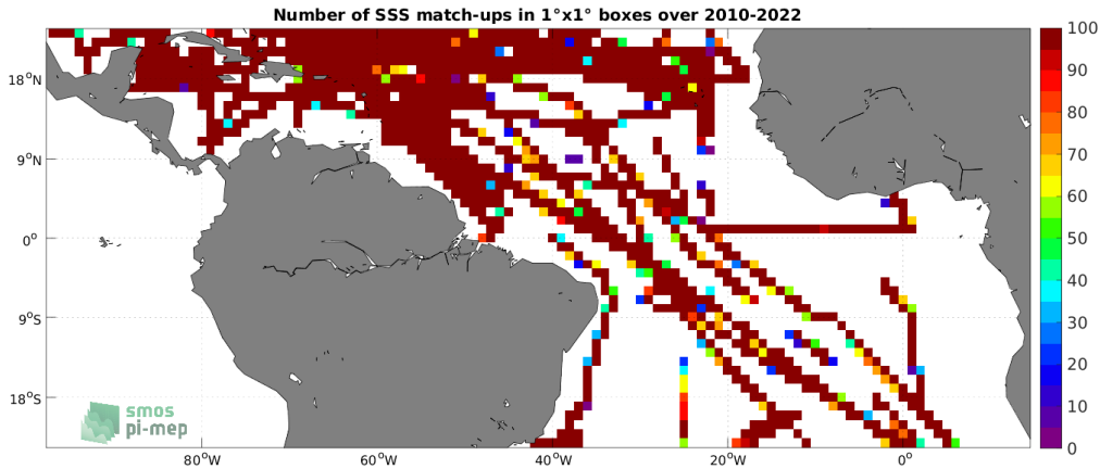
Figure 4: Number of SSS match-ups between TSG (SAMOS) SSS and the SMOS SSS L4 v1 - Monthly (CMEMS-CNR) SSS product for the Tropical Atlantic Ocean Pi-MEP region over 1^\circ \times 1^\circ boxes and for the full satellite product period.
