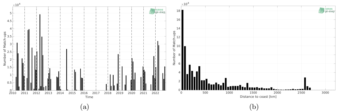
Figure 1: Number of match-ups between TSG (SAMOS) and SMOS SSS L4 v1 - Monthly (CMEMS-CNR) SSS as a function of time (a) and as function of the distance to coast (b) over the Tropical Atlantic Ocean Pi-MEP region and for the full satellite product period.
