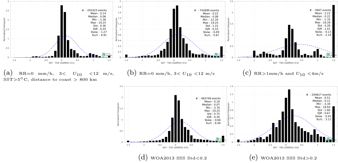
Figure 13: Normalized histogram of \Delta SSS (SMOS SSS L4 v1 - Monthly (CMEMS-CNR) - TSG (SAMOS)) for 5 different subdatasets corresponding to: RR=0 mm/h, 3 < U_{10} < 12 m/s, SST>5°C, distance to coast > 800 km (a), RR=0 mm/h, 3 < U_{10} < 12 m/s (b), RR>1mm/h and U_{10} < 4 m/s (c), WOA2013 SSS Std<0.2 (d), WOA2013 SSS Std>0.2 (e).
