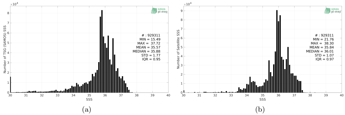
Figure 2: Histograms of SSS from TSG (SAMOS) (a) and SMOS SSS L4 v1 - Monthly (CMEMS-CNR) (b) considering all match-up pairs per bins of 0.1 over the Tropical Atlantic Ocean Pi-MEP region and for the full satellite product period.
