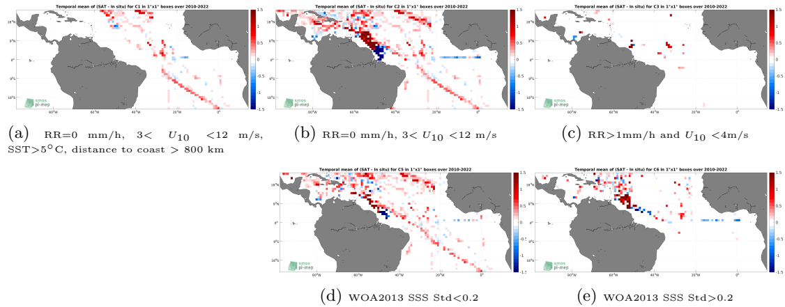
Figure 12: Temporal mean gridded over spatial boxes of size 1^\circ \times 1^\circ of \Delta\text{SSS} (SMOS SSS L4 v1 - Monthly (CMEMS-CNR) - TSG (SAMOS)) for 5 different subdatasets corresponding to:RR=0 mm/h, 3 < U_{10} < 12 m/s, SST >5^\circ\text{C} , distance to coast > 800 km (a), RR=0 mm/h, 3 < U_{10} < 12 m/s (b), RR >1 mm/h and U_{10} < 4 m/s (c), WOA2013 SSS Std <0.2 (d), WOA2013 SSS Std >0.2 (e).
