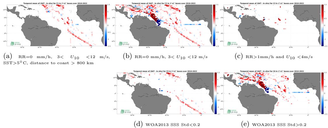
Figure 12: Temporal mean gridded over spatial boxes of size 1^\circ \times 1^\circ of \Delta SSS (SMOS SSS L4 v1 - Monthly (CMEMS-CNR) - TSG (SAMOS)) for 5 different subdatasets corresponding to:RR=0 mm/h, 3 < U_{10} < 12 m/s, SST >5^\circ\text{C} , distance to coast > 800 km (a), RR=0 mm/h, 3 < U_{10} < 12 m/s (b), RR >1 mm/h and U_{10} < 4 m/s (c), WOA2013 SSS Std <0.2 (d), WOA2013 SSS Std >0.2 (e).
