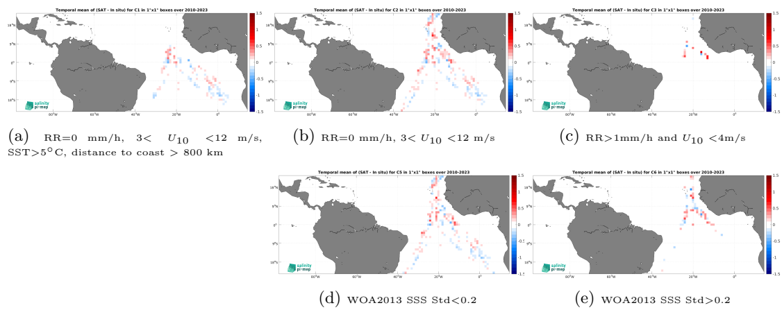
Figure 14: Temporal mean gridded over spatial boxes of size 1^\circ \times 1^\circ of \Delta SSS (SMOS SSS L4 v1 - Monthly (CMEMS-CNR) - TSG (Polarstern)) for 5 different subdatasets corresponding to:RR=0 mm/h, 3 < U_{10} < 12 m/s, SST >5^\circ\text{C} , distance to coast > 800 km (a), RR=0 mm/h, 3 < U_{10} < 12 m/s (b), RR >1 mm/h and U_{10} < 4 m/s (c), WOA2013 SSS Std <0.2 (d), WOA2013 SSS Std >0.2 (e).
