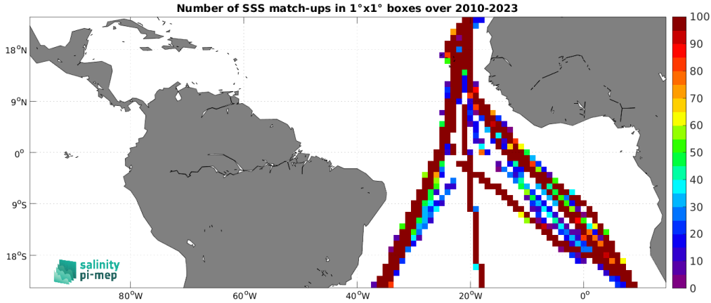
Figure 5: Number of SSS match-ups between TSG (Polarstern) SSS and the SMOS SSS L4 v1 - Monthly (CMEMS-CNR) SSS product for the Tropical Atlantic Ocean Pi-MEP region over 1^\circ \times 1^\circ boxes and for the full satellite product period.
