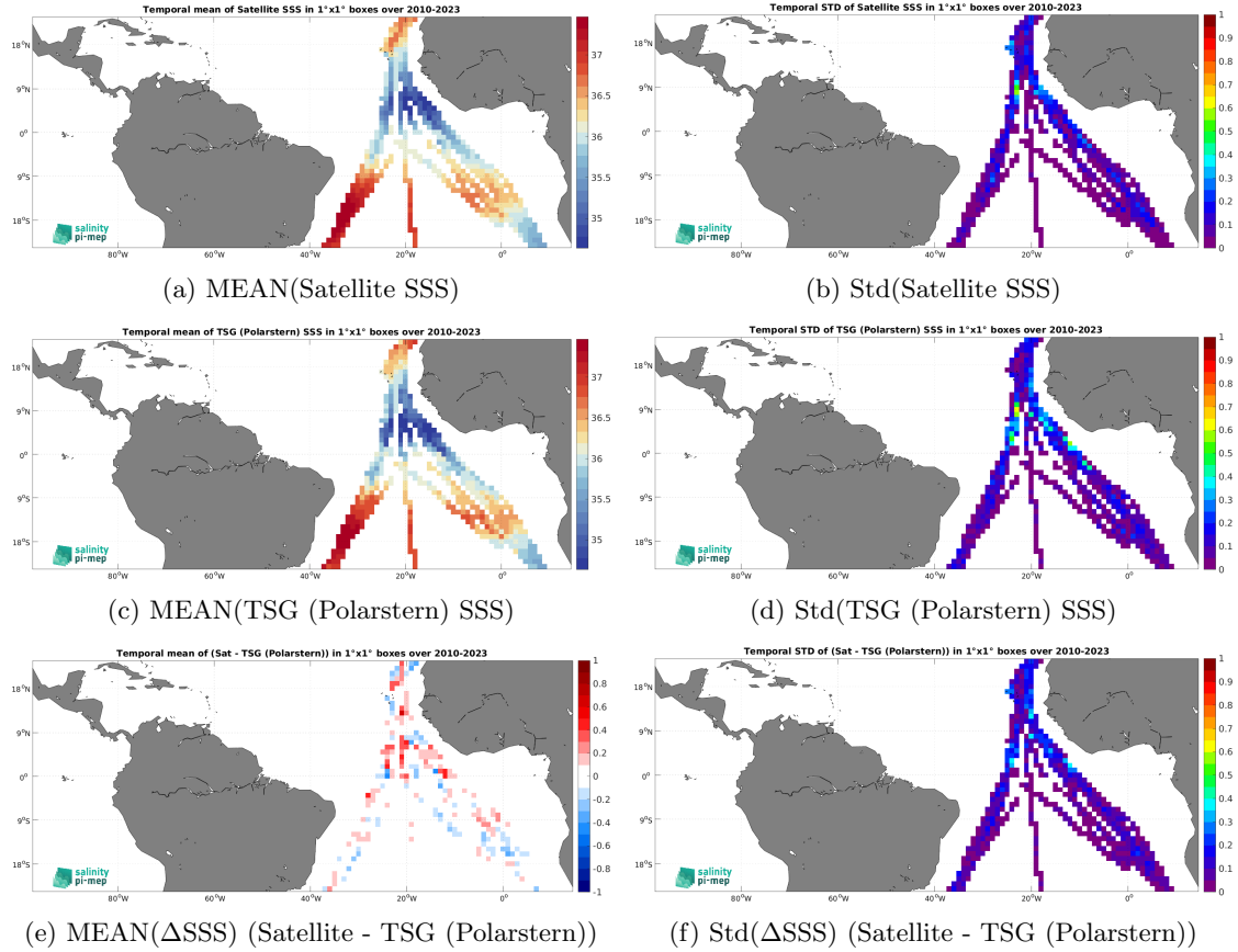
Figure 7: Temporal mean (left) and Std (right) of SSS from SMOS SSS L4 v1 - Monthly (CMEMS-CNR) (top), TSG (Polarstern) (middle), and of \Delta\text{SSS} (Satellite - TSG (Polarstern)). Only match-up pairs are used to generate these maps.
