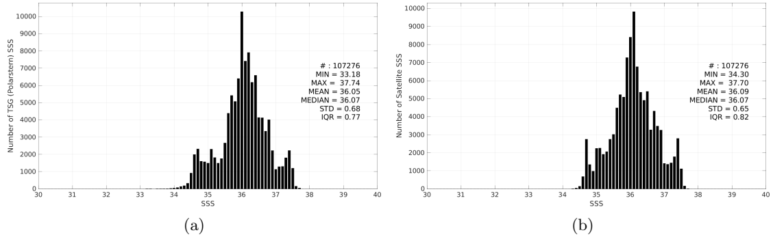
Figure 3: Histograms of SSS from TSG (Polarstern) (a) and SMOS SSS L4 v1 - Monthly (CMEMS-CNR) (b) considering all match-up pairs per bins of 0.1 over the Tropical Atlantic Ocean Pi-MEP region and for the full satellite product period.
