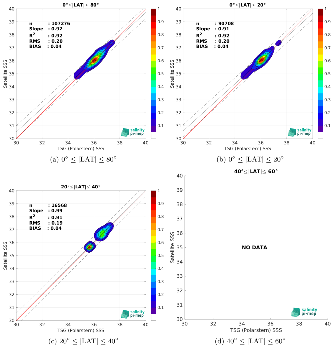
Figure 10: Contour maps of the concentration of SMOS SSS L4 v1 - Monthly (CMEMS-CNR) SSS (y-axis) versus TSG (Polarstern) SSS (x-axis) at match-up pairs for different latitude bands. For each plot, the red line shows x=y . The black thin and dashed lines indicate a linear fit through the data cloud and the \pm 95\% confidence levels, respectively. The number match-up pairs n , the slope and R^2 coefficient of the linear fit, the root mean square (RMS) and the mean bias between satellite and in situ data are indicated for each latitude band in each plots.
