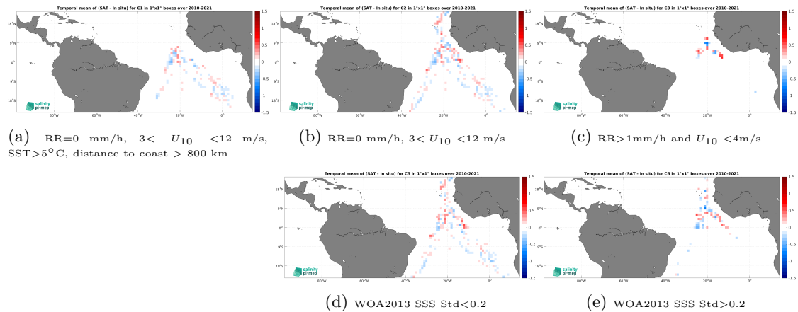
Figure 12: Temporal mean gridded over spatial boxes of size 1^\circ \times 1^\circ of \Delta\text{SSS} (SMOS SSS L4 v1 - Monthly (CMEMS-CNR) - TSG (Polarstern)) for 5 different subdatasets corresponding to:RR=0 mm/h, 3 < U_{10} < 12 m/s, SST >5^\circ\text{C} , distance to coast > 800 km (a), RR=0 mm/h, 3 < U_{10} < 12 m/s (b), RR >1 mm/h and U_{10} < 4 m/s (c), WOA2013 SSS Std <0.2 (d), WOA2013 SSS Std >0.2 (e).
