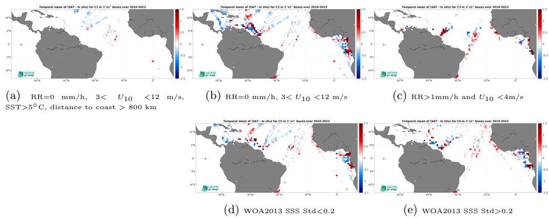
Figure 14: Temporal mean gridded over spatial boxes of size 1^\circ \times 1^\circ of \Delta\text{SSS} (SMOS SSS L4 v1 - Monthly (CMEMS-CNR) - TSG (LEGOS-DM)) for 5 different subdatasets corresponding to:RR=0 mm/h, 3 < U_{10} < 12 m/s, SST >5^\circ\text{C} , distance to coast > 800 km (a), RR=0 mm/h, 3 < U_{10} < 12 m/s (b), RR >1 mm/h and U_{10} < 4 m/s (c), WOA2013 SSS Std <0.2 (d), WOA2013 SSS Std >0.2 (e).
