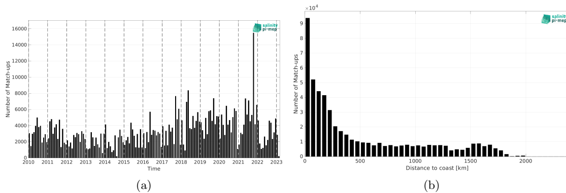
Figure 2: Number of match-ups between TSG (LEGOS-DM) and SMOS SSS L4 v1 - Monthly (CMEMS-CNR) SSS as a function of time (a) and as function of the distance to coast (b) over the Tropical Atlantic Ocean Pi-MEP region and for the full satellite product period.
