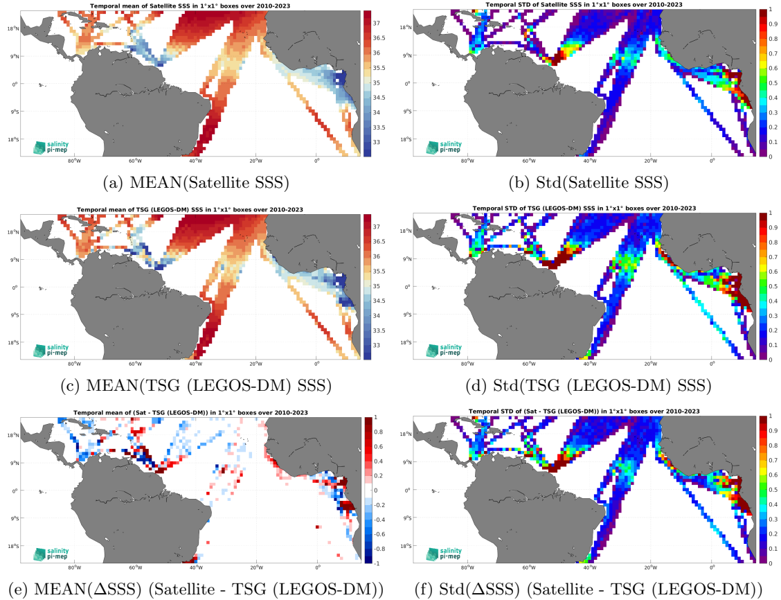
Figure 7: Temporal mean (left) and Std (right) of SSS from SMOS SSS L4 v1 - Monthly (CMEMS-CNR) (top), TSG (LEGOS-DM) (middle), and of \Delta\text{SSS} (Satellite - TSG (LEGOS-DM)). Only match-up pairs are used to generate these maps.
