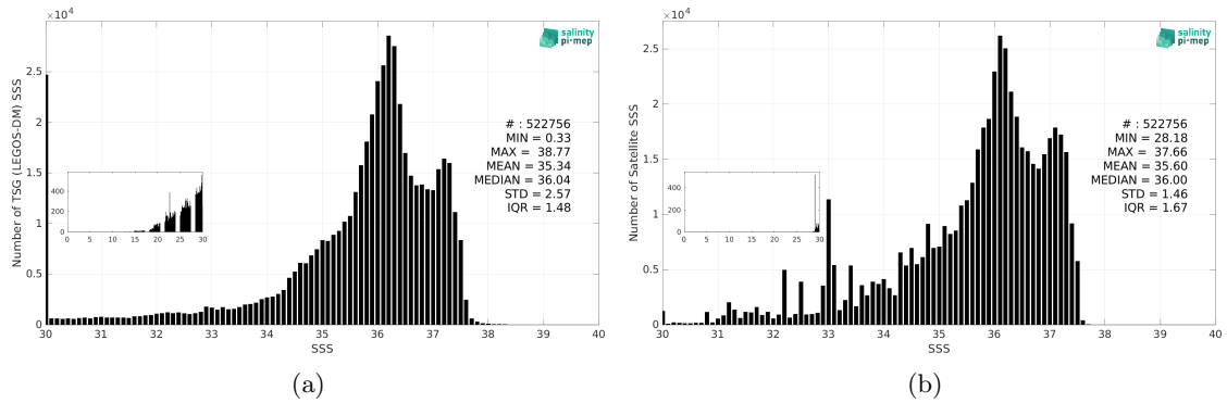
Figure 3: Histograms of SSS from TSG (LEGOS-DM) (a) and SMOS SSS L4 v1 - Monthly (CMEMS-CNR) (b) considering all match-up pairs per bins of 0.1 over the Tropical Atlantic Ocean Pi-MEP region and for the full satellite product period.
