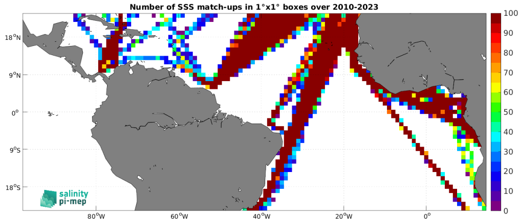
Figure 5: Number of SSS match-ups between TSG (LEGOS-DM) SSS and the SMOS SSS L4 v1 - Monthly (CMEMS-CNR) SSS product for the Tropical Atlantic Ocean Pi-MEP region over 1^\circ \times 1^\circ boxes and for the full satellite product period.
