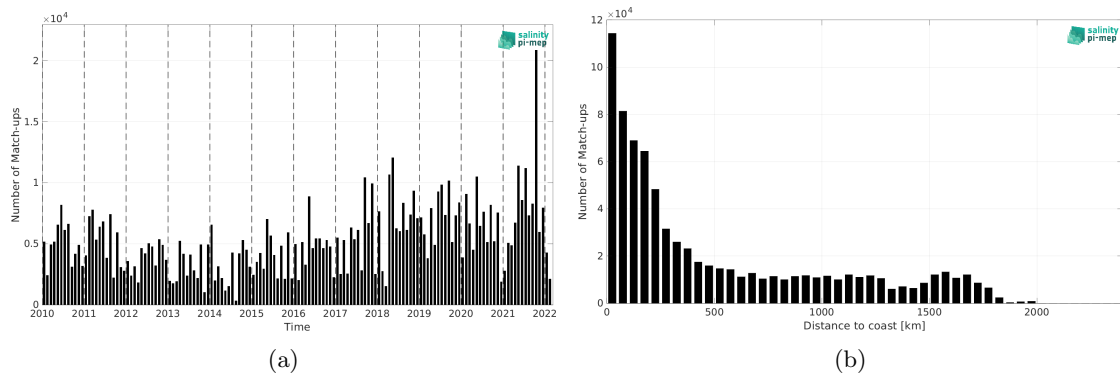
Figure 1: Number of match-ups between TSG (LEGOS-DM) and SMOS SSS L4 v1 - Monthly (CMEMS-CNR) SSS as a function of time (a) and as function of the distance to coast (b) over the Tropical Atlantic Ocean Pi-MEP region and for the full satellite product period.
