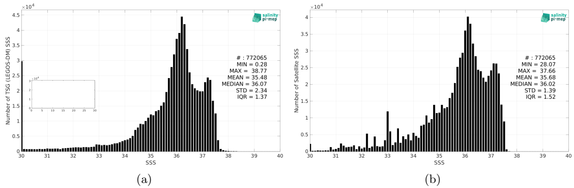
Figure 2: Histograms of SSS from TSG (LEGOS-DM) (a) and SMOS SSS L4 v1 - Monthly (CMEMS-CNR) (b) considering all match-up pairs per bins of 0.1 over the Tropical Atlantic Ocean Pi-MEP region and for the full satellite product period.
