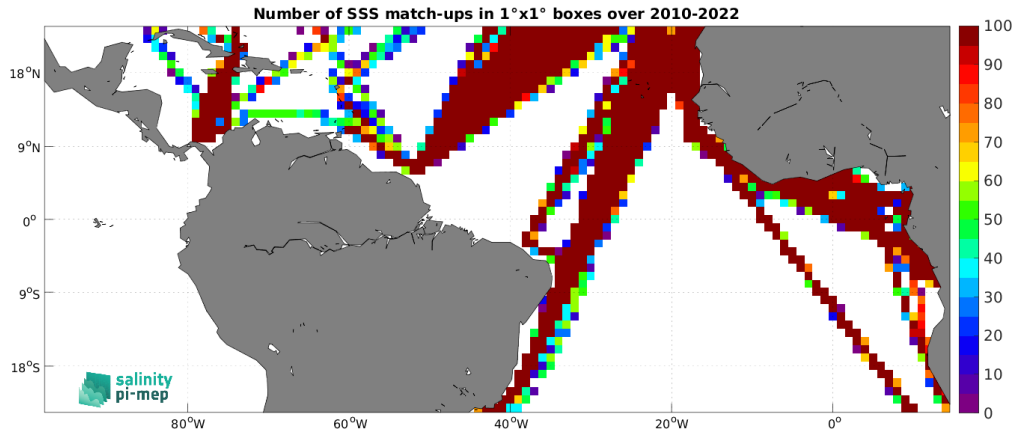
Figure 4: Number of SSS match-ups between TSG (LEGOS-DM) SSS and the SMOS SSS L4 v1 - Monthly (CMEMS-CNR) SSS product for the Tropical Atlantic Ocean Pi-MEP region over 1^\circ \times 1^\circ boxes and for the full satellite product period.
