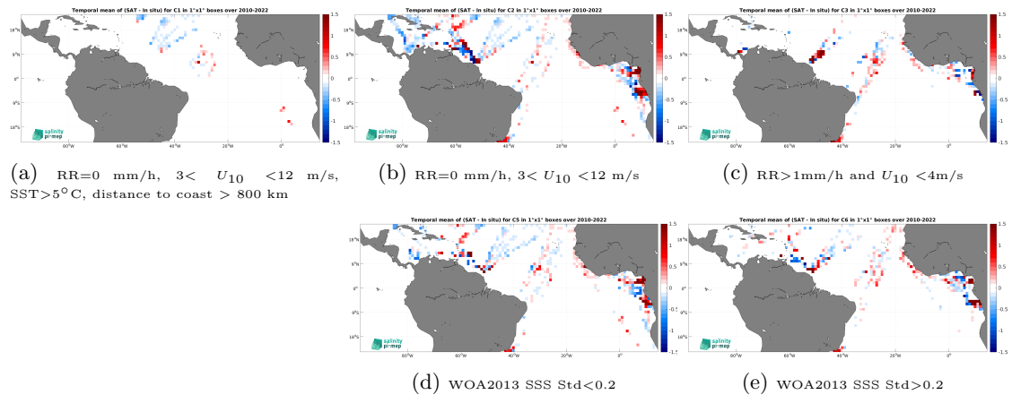
Figure 12: Temporal mean gridded over spatial boxes of size 1^\circ \times 1^\circ of \Delta\text{SSS} (SMOS SSS L4 v1 - Monthly (CMEMS-CNR) - TSG (LEGOS-DM)) for 5 different subdatasets corresponding to:RR=0 mm/h, 3 < U_{10} < 12 m/s, SST >5^\circ\text{C} , distance to coast > 800 km (a), RR=0 mm/h, 3 < U_{10} < 12 m/s (b), RR >1 mm/h and U_{10} < 4 m/s (c), WOA2013 SSS Std <0.2 (d), WOA2013 SSS Std >0.2 (e).
