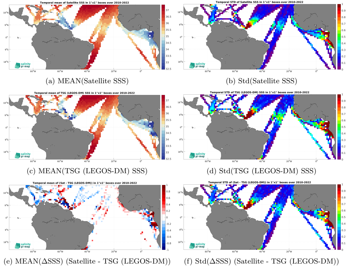
Figure 6: Temporal mean (left) and Std (right) of SSS from SMOS SSS L4 v1 - Monthly (CMEMS-CNR) (top), TSG (LEGOS-DM) (middle), and of \Delta\text{SSS} (Satellite - TSG (LEGOS-DM)). Only match-up pairs are used to generate these maps.
