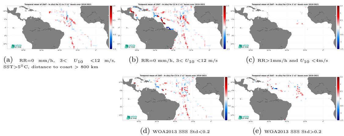
Figure 14: Temporal mean gridded over spatial boxes of size 1^\circ \times 1^\circ of \Delta\text{SSS} (SMOS SSS L4 v1 - Monthly (CMEMS-CNR) - TSG (GOSUD-Sailing-ship)) for 5 different subdatasets corresponding to:RR=0 mm/h, 3 < U_{10} < 12 m/s, SST >5^\circ\text{C} , distance to coast > 800 km (a), RR=0 mm/h, 3 < U_{10} < 12 m/s (b), RR >1 mm/h and U_{10} < 4 m/s (c), WOA2013 SSS Std <0.2 (d), WOA2013 SSS Std >0.2 (e).
