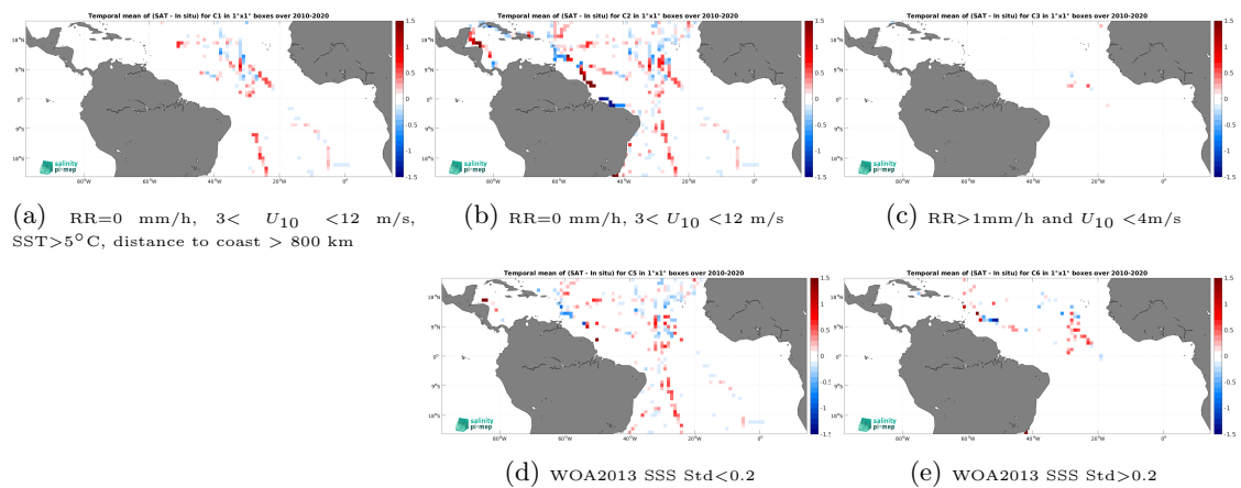
Figure 14: Temporal mean gridded over spatial boxes of size 1^\circ \times 1^\circ of \Delta\text{SSS} (SMOS SSS L4 v1 - Monthly (CMEMS-CNR) - TSG (GOSUD-Sailing-ship)) for 5 different subdatasets corresponding to:RR=0 mm/h, 3 < U_{10} < 12 m/s, SST>5°C, distance to coast > 800 km (a), RR=0 mm/h, 3 < U_{10} < 12 m/s (b), RR>1mm/h and U_{10} < 4 m/s (c), WOA2013 SSS Std<0.2 (d), WOA2013 SSS Std>0.2 (e).
