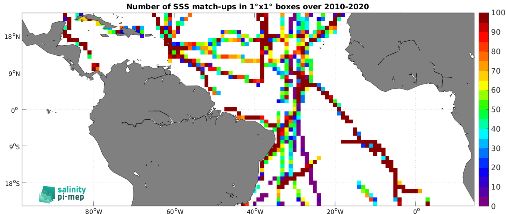
Figure 5: Number of SSS match-ups between TSG (GOSUD-Sailing-ship) SSS and the SMOS SSS L4 v1 - Monthly (CMEMS-CNR) SSS product for the Tropical Atlantic Ocean Pi-MEP region over 1^\circ \times 1^\circ boxes and for the full satellite product period.
