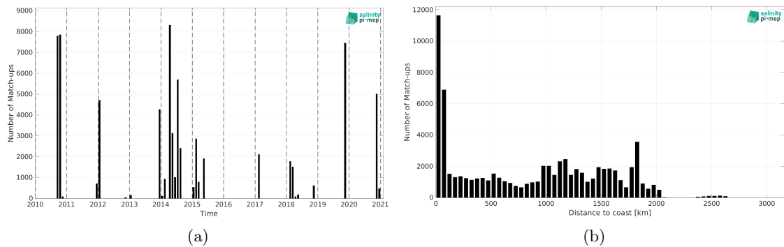
Figure 2: Number of match-ups between TSG (GOSUD-Sailing-ship) and SMOS SSS L4 v1 - Monthly (CMEMS-CNR) SSS as a function of time (a) and as function of the distance to coast (b) over the Tropical Atlantic Ocean Pi-MEP region and for the full satellite product period.
