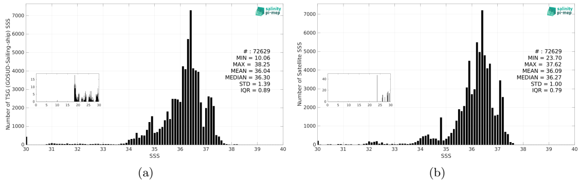
Figure 3: Histograms of SSS from TSG (GOSUD-Sailing-ship) (a) and SMOS SSS L4 v1 - Monthly (CMEMS-CNR) (b) considering all match-up pairs per bins of 0.1 over the Tropical Atlantic Ocean Pi-MEP region and for the full satellite product period.
