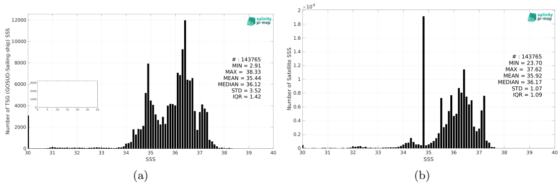
Figure 2: Histograms of SSS from TSG (GOSUD-Sailing-ship) (a) and SMOS SSS L4 v1 - Monthly (CMEMS-CNR) (b) considering all match-up pairs per bins of 0.1 over the Tropical Atlantic Ocean Pi-MEP region and for the full satellite product period.
