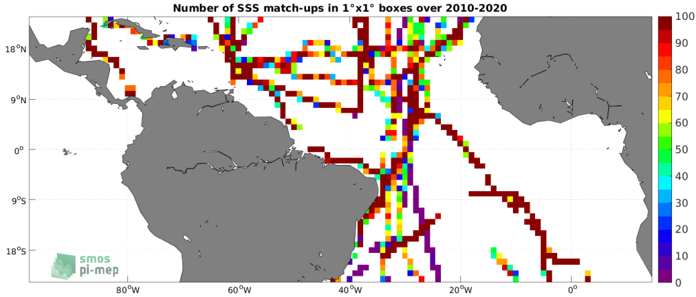
Figure 4: Number of SSS match-ups between TSG (GOSUD-Sailing-ship) SSS and the SMOS SSS L4 v1 - Monthly (CMEMS-CNR) SSS product for the Tropical Atlantic Ocean Pi-MEP region over 1^\circ \times 1^\circ boxes and for the full satellite product period.
