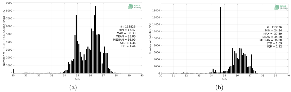
Figure 2: Histograms of SSS from TSG (GOSUD-Sailing-ship) (a) and SMOS SSS L4 v1 - Monthly (CMEMS-CNR) (b) considering all match-up pairs per bins of 0.1 over the Tropical Atlantic Ocean Pi-MEP region and for the full satellite product period.
