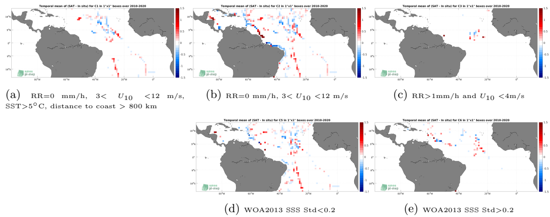
Figure 12: Temporal mean gridded over spatial boxes of size 1^\circ \times 1^\circ of \Delta\text{SSS} (SMOS SSS L4 v1 - Monthly (CMEMS-CNR) - TSG (GOSUD-Sailing-ship)) for 5 different subdatasets corresponding to:RR=0 mm/h, 3 < U_{10} < 12 m/s, SST >5^\circ\text{C} , distance to coast > 800 km (a), RR=0 mm/h, 3 < U_{10} < 12 m/s (b), RR >1 mm/h and U_{10} < 4 m/s (c), WOA2013 SSS Std <0.2 (d), WOA2013 SSS Std >0.2 (e).
