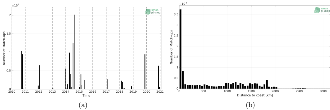
Figure 1: Number of match-ups between TSG (GOSUD-Sailing-ship) and SMOS SSS L4 v1 - Monthly (CMEMS-CNR) SSS as a function of time (a) and as function of the distance to coast (b) over the Tropical Atlantic Ocean Pi-MEP region and for the full satellite product period.
