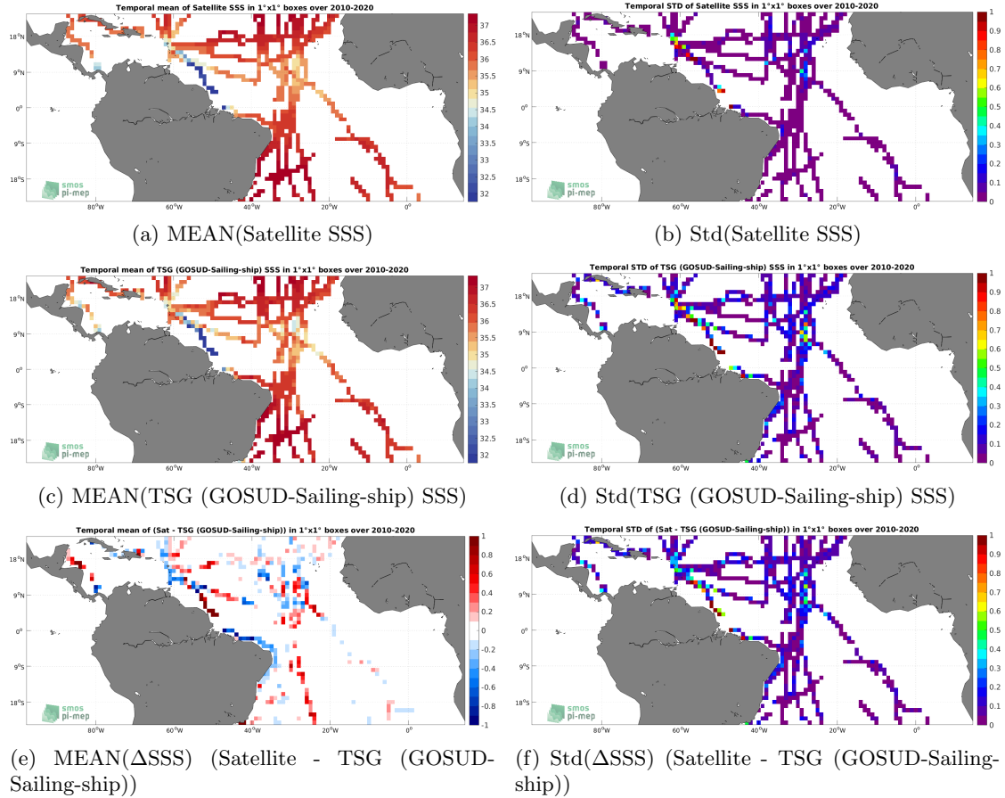
Figure 6: Temporal mean (left) and Std (right) of SSS from SMOS SSS L4 v1 - Monthly (CMEMS-CNR) (top), TSG (GOSUD-Sailing-ship) (middle), and of \Delta\text{SSS} (Satellite - TSG (GOSUD-Sailing-ship)). Only match-up pairs are used to generate these maps.
