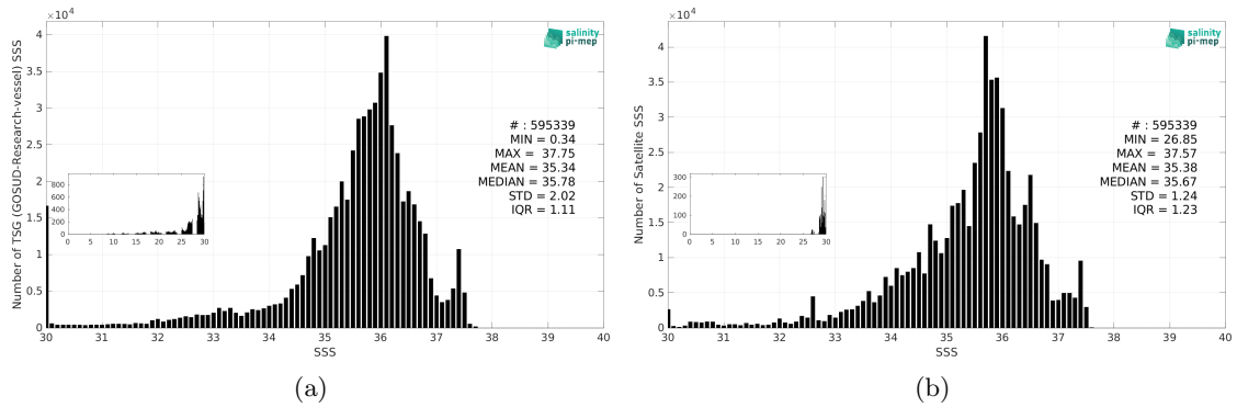
Figure 3: Histograms of SSS from TSG (GOSUD-Research-vessel) (a) and SMOS SSS L4 v1 - Monthly (CMEMS-CNR) (b) considering all match-up pairs per bins of 0.1 over the Tropical Atlantic Ocean Pi-MEP region and for the full satellite product period.
