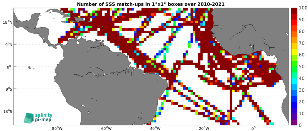
Figure 5: Number of SSS match-ups between TSG (GOSUD-Research-vessel) SSS and the SMOS SSS L4 v1 - Monthly (CMEMS-CNR) SSS product for the Tropical Atlantic Ocean Pi-MEP region over 1^\circ \times 1^\circ boxes and for the full satellite product period.
