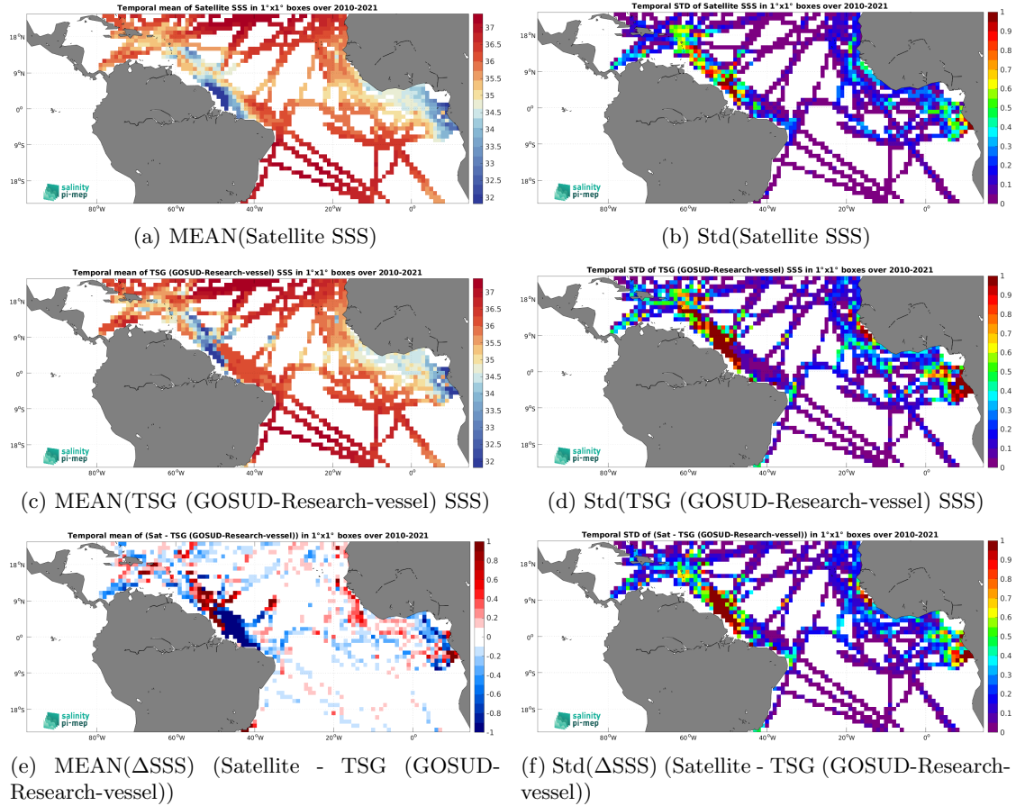
Figure 7: Temporal mean (left) and Std (right) of SSS from SMOS SSS L4 v1 - Monthly (CMEMS-CNR) (top), TSG (GOSUD-Research-vessel) (middle), and of \Delta\text{SSS} (Satellite - TSG (GOSUD-Research-vessel)). Only match-up pairs are used to generate these maps.
