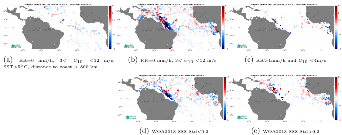
Figure 14: Temporal mean gridded over spatial boxes of size 1^\circ \times 1^\circ of \Delta\text{SSS} (SMOS SSS L4 v1 - Monthly (CMEMS-CNR) - TSG (GOSUD-Research-vessel)) for 5 different subdatasets corresponding to:RR=0 mm/h, 3 < U_{10} < 12 m/s, SST >5^\circ\text{C} , distance to coast > 800 km (a), RR=0 mm/h, 3 < U_{10} < 12 m/s (b), RR >1 mm/h and U_{10} < 4 m/s (c), WOA2013 SSS Std <0.2 (d), WOA2013 SSS Std >0.2 (e).
