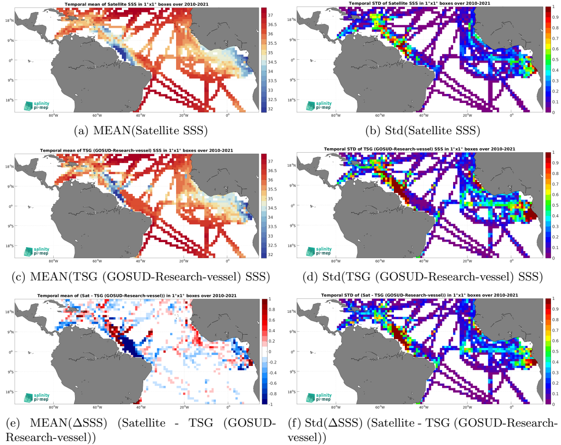
Figure 6: Temporal mean (left) and Std (right) of SSS from SMOS SSS L4 v1 - Monthly (CMEMS-CNR) (top), TSG (GOSUD-Research-vessel) (middle), and of \Delta\text{SSS} (Satellite - TSG (GOSUD-Research-vessel)). Only match-up pairs are used to generate these maps.
