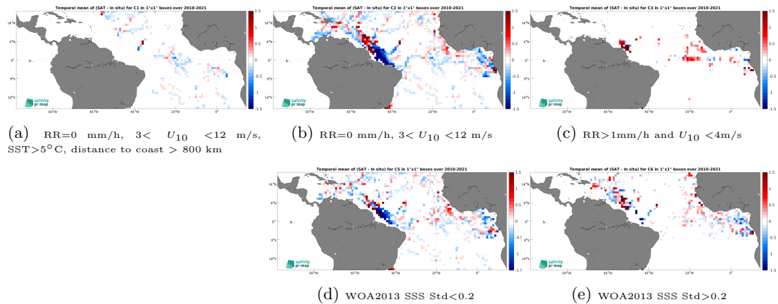
Figure 12: Temporal mean gridded over spatial boxes of size 1^\circ \times 1^\circ of \Delta SSS (SMOS SSS L4 v1 - Monthly (CMEMS-CNR) - TSG (GOSUD-Research-vessel)) for 5 different subdatasets corresponding to:RR=0 mm/h, 3 < U_{10} < 12 m/s, SST >5^\circ\text{C} , distance to coast > 800 km (a), RR=0 mm/h, 3 < U_{10} < 12 m/s (b), RR >1 mm/h and U_{10} < 4 m/s (c), WOA2013 SSS Std <0.2 (d), WOA2013 SSS Std >0.2 (e).
