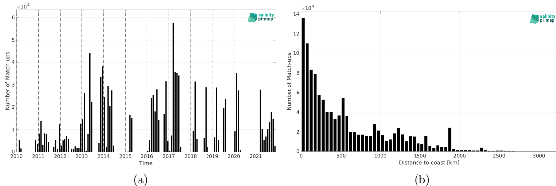
Figure 1: Number of match-ups between TSG (GOSUD-Research-vessel) and SMOS SSS L4 v1 - Monthly (CMEMS-CNR) SSS as a function of time (a) and as function of the distance to coast (b) over the Tropical Atlantic Ocean Pi-MEP region and for the full satellite product period.
