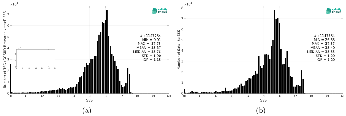
Figure 2: Histograms of SSS from TSG (GOSUD-Research-vessel) (a) and SMOS SSS L4 v1 - Monthly (CMEMS-CNR) (b) considering all match-up pairs per bins of 0.1 over the Tropical Atlantic Ocean Pi-MEP region and for the full satellite product period.
