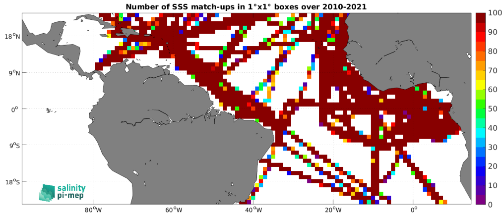
Figure 4: Number of SSS match-ups between TSG (GOSUD-Research-vessel) SSS and the SMOS SSS L4 v1 - Monthly (CMEMS-CNR) SSS product for the Tropical Atlantic Ocean Pi-MEP region over 1^\circ \times 1^\circ boxes and for the full satellite product period.
