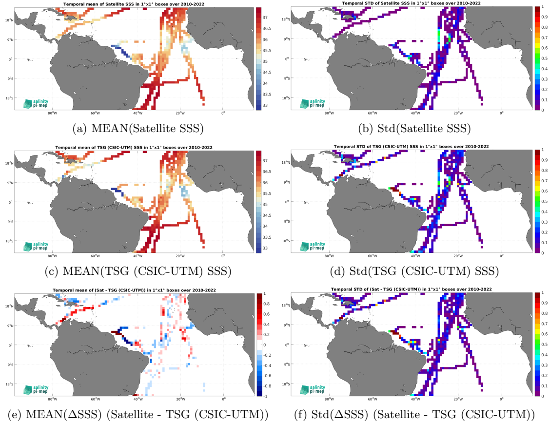
Figure 7: Temporal mean (left) and Std (right) of SSS from SMOS SSS L4 v1 - Monthly (CMEMS-CNR) (top), TSG (CSIC-UTM) (middle), and of \Delta\text{SSS} (Satellite - TSG (CSIC-UTM)). Only match-up pairs are used to generate these maps.
