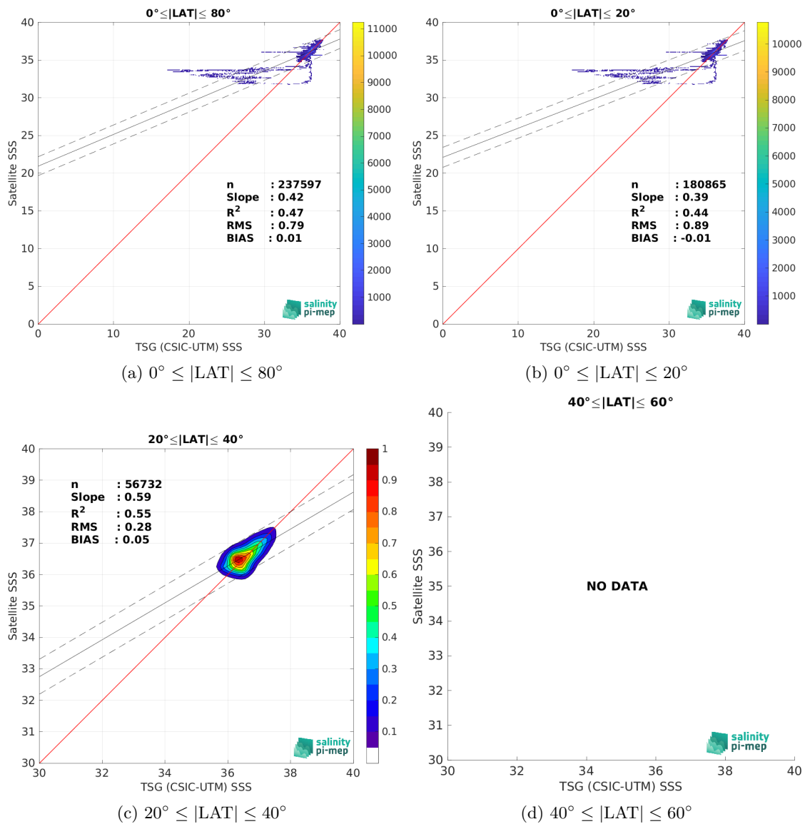
Figure 10: Contour maps of the concentration of SMOS SSS L4 v1 - Monthly (CMEMS-CNR) SSS (y-axis) versus TSG (CSIC-UTM) SSS (x-axis) at match-up pairs for different latitude bands. For each plot, the red line shows x=y . The black thin and dashed lines indicate a linear fit through the data cloud and the \pm 95\% confidence levels, respectively. The number match-up pairs n , the slope and R^2 coefficient of the linear fit, the root mean square (RMS) and the mean bias between satellite and in situ data are indicated for each latitude band in each plots.
