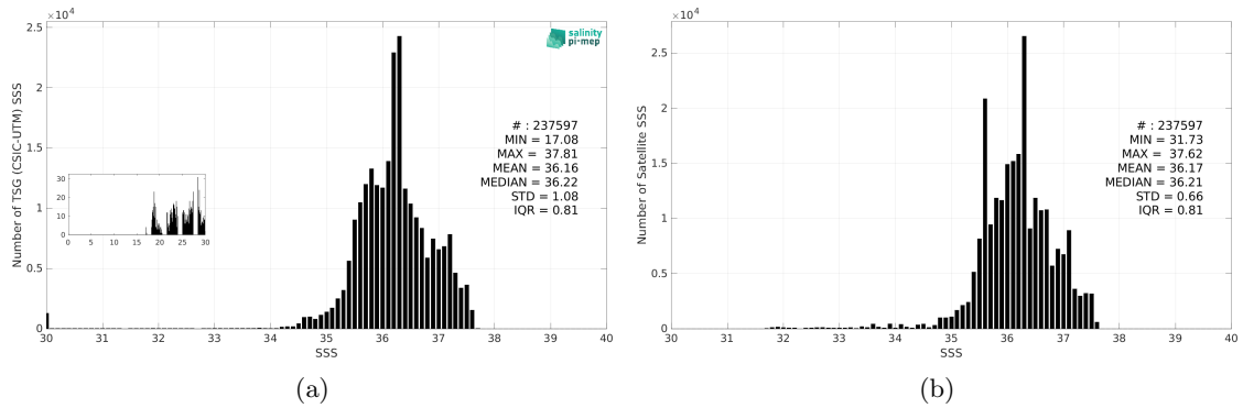
Figure 3: Histograms of SSS from TSG (CSIC-UTM) (a) and SMOS SSS L4 v1 - Monthly (CMEMS-CNR) (b) considering all match-up pairs per bins of 0.1 over the Tropical Atlantic Ocean Pi-MEP region and for the full satellite product period.
