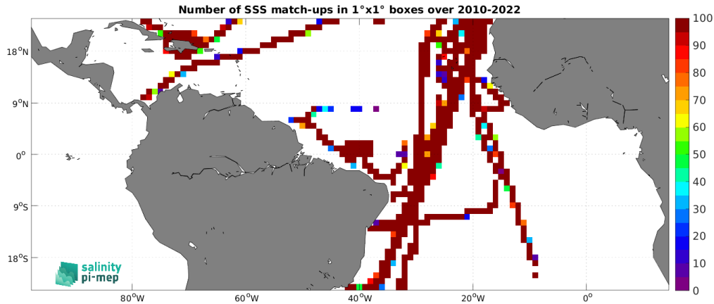
Figure 5: Number of SSS match-ups between TSG (CSIC-UTM) SSS and the SMOS SSS L4 v1 - Monthly (CMEMS-CNR) SSS product for the Tropical Atlantic Ocean Pi-MEP region over 1^\circ \times 1^\circ boxes and for the full satellite product period.
