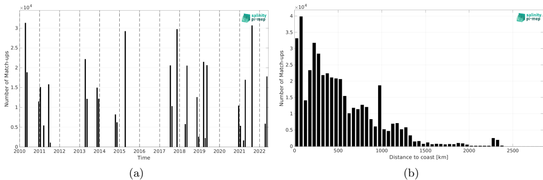
Figure 1: Number of match-ups between TSG (CSIC-UTM) and SMOS SSS L4 v1 - Monthly (CMEMS-CNR) SSS as a function of time (a) and as function of the distance to coast (b) over the Tropical Atlantic Ocean Pi-MEP region and for the full satellite product period.
