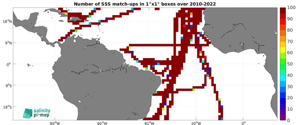
Figure 4: Number of SSS match-ups between TSG (CSIC-UTM) SSS and the SMOS SSS L4 v1 - Monthly (CMEMS-CNR) SSS product for the Tropical Atlantic Ocean Pi-MEP region over 1^\circ \times 1^\circ boxes and for the full satellite product period.
