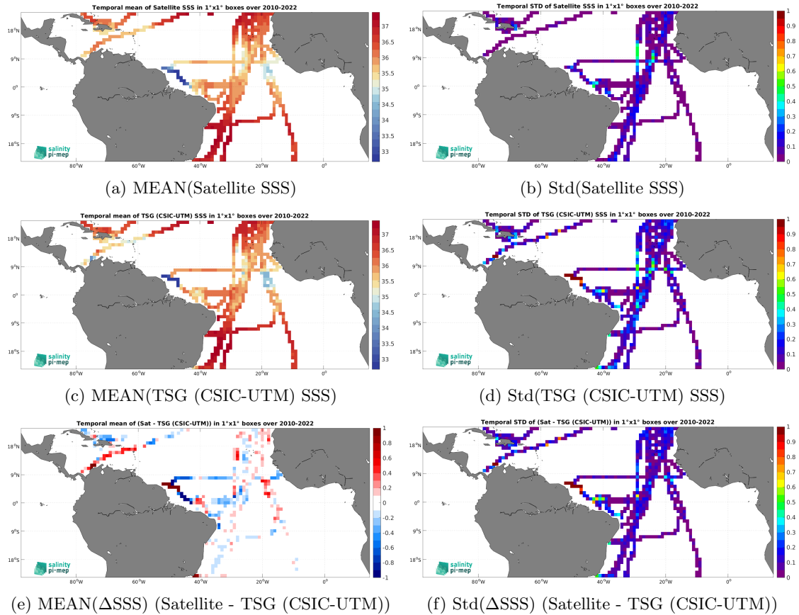
Figure 6: Temporal mean (left) and Std (right) of SSS from SMOS SSS L4 v1 - Monthly (CMEMS-CNR) (top), TSG (CSIC-UTM) (middle), and of \Delta\text{SSS} (Satellite - TSG (CSIC-UTM)). Only match-up pairs are used to generate these maps.
