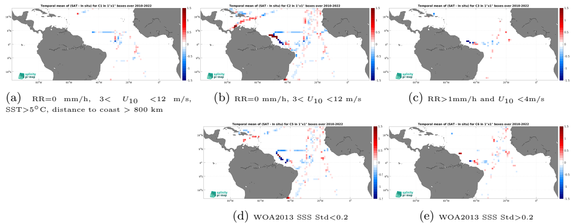
Figure 12: Temporal mean gridded over spatial boxes of size 1^\circ \times 1^\circ of \Delta\text{SSS} (SMOS SSS L4 v1 - Monthly (CMEMS-CNR) - TSG (CSIC-UTM)) for 5 different subdatasets corresponding to:RR=0 mm/h, 3 < U_{10} < 12 m/s, SST >5^\circ\text{C} , distance to coast > 800 km (a), RR=0 mm/h, 3 < U_{10} < 12 m/s (b), RR >1 mm/h and U_{10} < 4 m/s (c), WOA2013 SSS Std <0.2 (d), WOA2013 SSS Std >0.2 (e).
