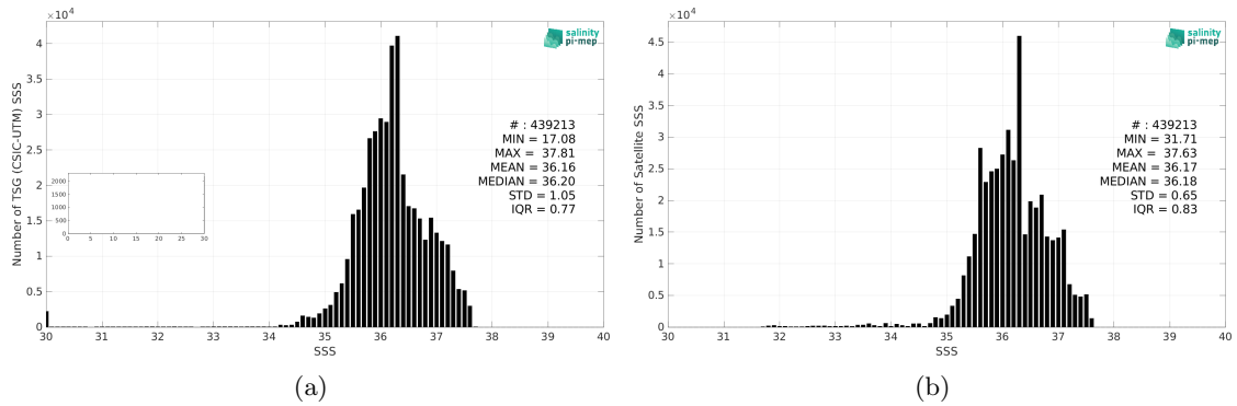
Figure 2: Histograms of SSS from TSG (CSIC-UTM) (a) and SMOS SSS L4 v1 - Monthly (CMEMS-CNR) (b) considering all match-up pairs per bins of 0.1 over the Tropical Atlantic Ocean Pi-MEP region and for the full satellite product period.
