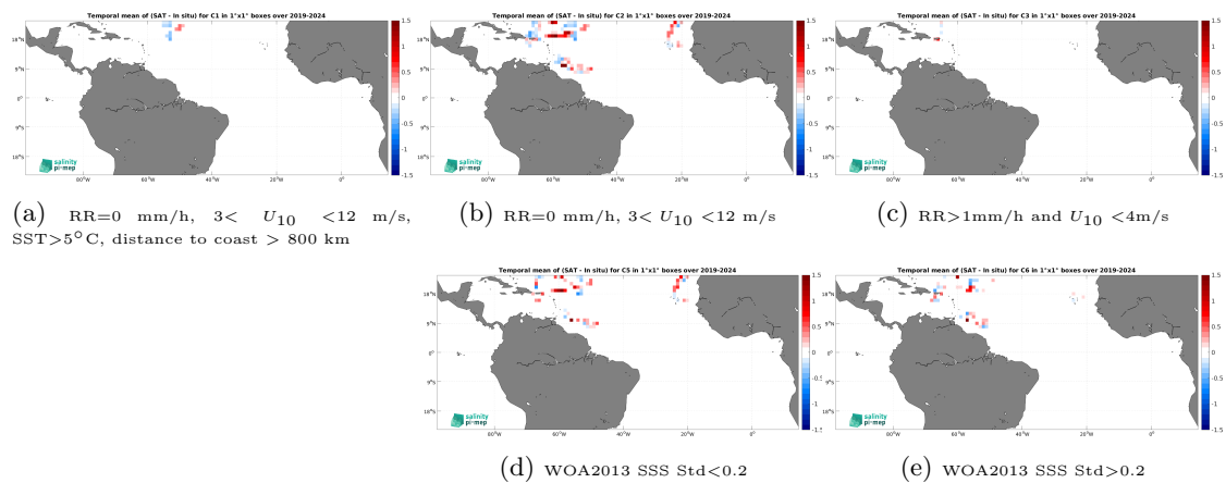
Figure 14: Temporal mean gridded over spatial boxes of size 1^\circ \times 1^\circ of \Delta\text{SSS} (SMOS SSS L4 v1 - Monthly (CMEMS-CNR) - Saildrone) for 5 different subdatasets corresponding to:RR=0 mm/h, 3 < U_{10} < 12 m/s, SST >5^\circ\text{C} , distance to coast > 800 km (a), RR=0 mm/h, 3 < U_{10} < 12 m/s (b), RR >1 mm/h and U_{10} < 4 m/s (c), WOA2013 SSS Std <0.2 (d), WOA2013 SSS Std >0.2 (e).
