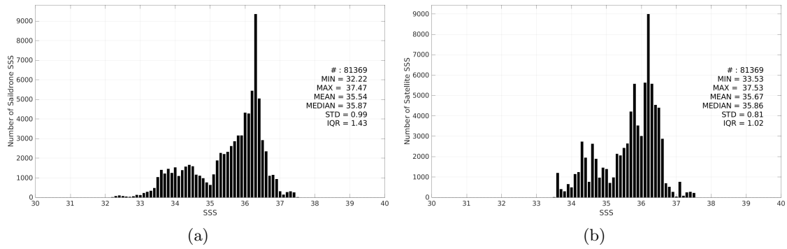
Figure 3: Histograms of SSS from Saildrone (a) and SMOS SSS L4 v1 - Monthly (CMEMS-CNR) (b) considering all match-up pairs per bins of 0.1 over the Tropical Atlantic Ocean Pi-MEP region and for the full satellite product period.
