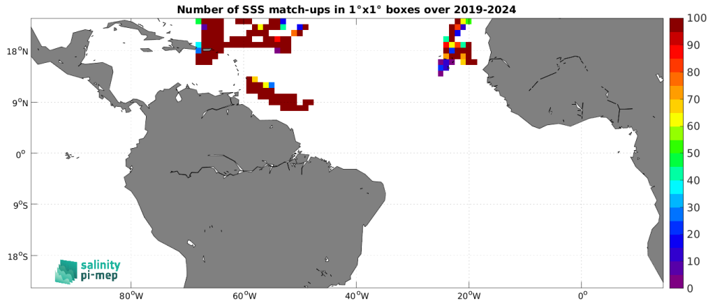
Figure 5: Number of SSS match-ups between Saildrone SSS and the SMOS SSS L4 v1 - Monthly (CMEMS-CNR) SSS product for the Tropical Atlantic Ocean Pi-MEP region over 1^\circ \times 1^\circ boxes and for the full satellite product period.
