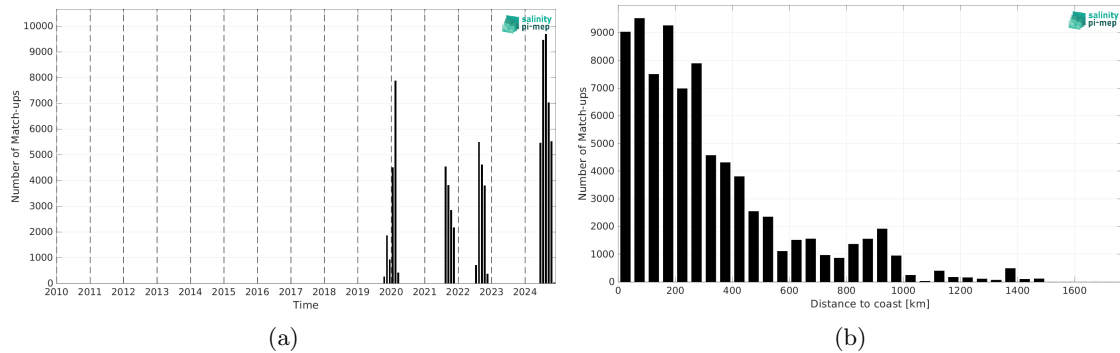
Figure 2: Number of match-ups between Saildrone and SMOS SSS L4 v1 - Monthly (CMEMS-CNR) SSS as a function of time (a) and as function of the distance to coast (b) over the Tropical Atlantic Ocean Pi-MEP region and for the full satellite product period.
