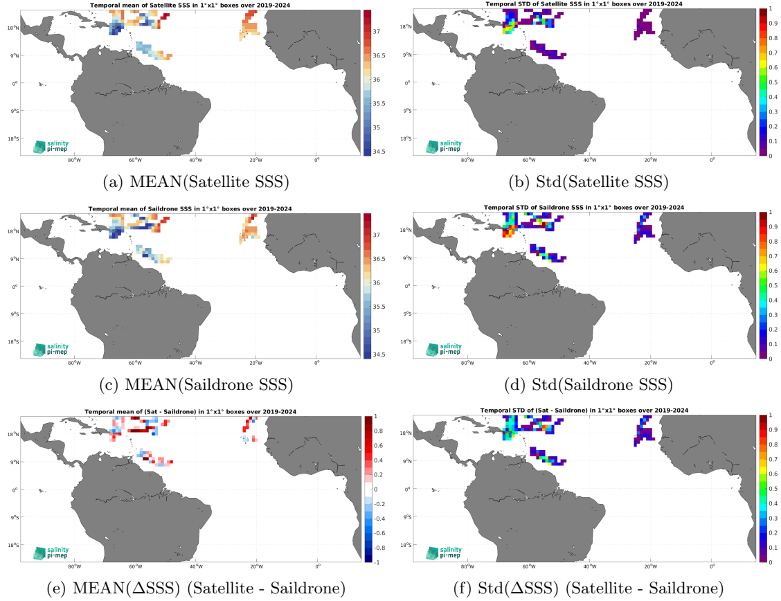
Figure 7: Temporal mean (left) and Std (right) of SSS from SMOS SSS L4 v1 - Monthly (CMEMS-CNR) (top), Saildrone (middle), and of \Delta\text{SSS} (Satellite - Saildrone). Only match-up pairs are used to generate these maps.
