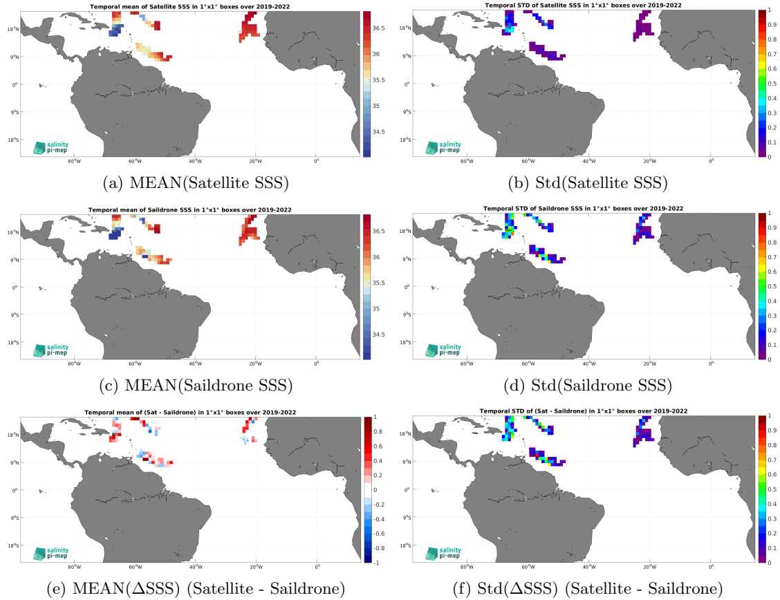
Figure 7: Temporal mean (left) and Std (right) of SSS from SMOS SSS L4 v1 - Monthly (CMEMS-CNR) (top), Sairdrone (middle), and of \Delta SSS (Satellite - Sairdrone). Only match-up pairs are used to generate these maps.
