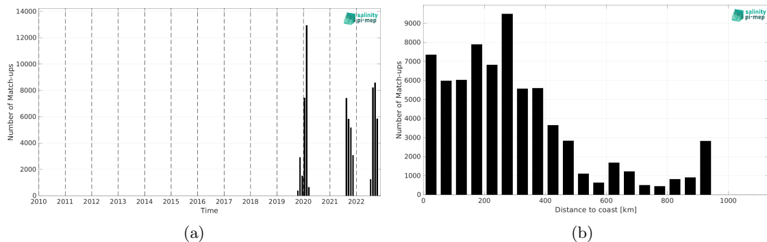
Figure 1: Number of match-ups between Saildrone and SMOS SSS L4 v1 - Monthly (CMEMS-CNR) SSS as a function of time (a) and as function of the distance to coast (b) over the Tropical Atlantic Ocean Pi-MEP region and for the full satellite product period.
