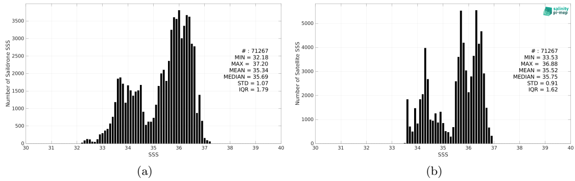
Figure 2: Histograms of SSS from Saildrone (a) and SMOS SSS L4 v1 - Monthly (CMEMS-CNR) (b) considering all match-up pairs per bins of 0.1 over the Tropical Atlantic Ocean Pi-MEP region and for the full satellite product period.
