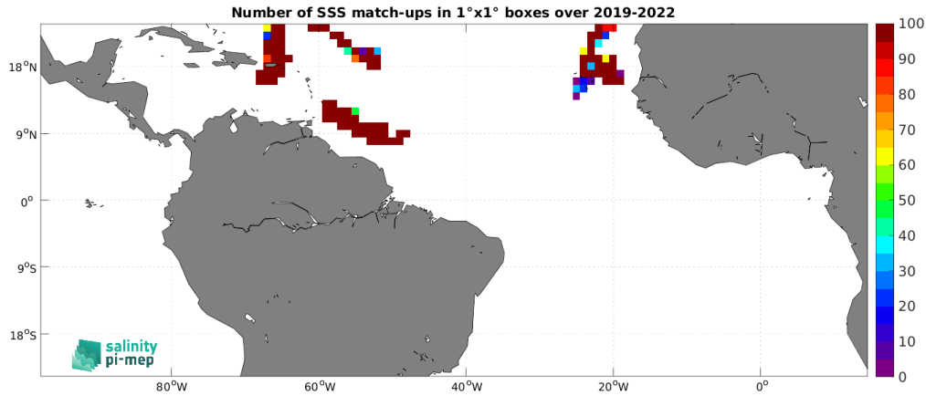
Figure 4: Number of SSS match-ups between Saildrone SSS and the SMOS SSS L4 v1 - Monthly (CMEMS-CNR) SSS product for the Tropical Atlantic Ocean Pi-MEP region over 1^\circ \times 1^\circ boxes and for the full satellite product period.
