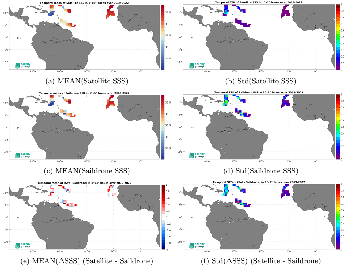
Figure 6: Temporal mean (left) and Std (right) of SSS from SMOS SSS L4 v1 - Monthly (CMEMS-CNR) (top), Sairdrone (middle), and of \Delta\text{SSS} (Satellite - Sairdrone). Only match-up pairs are used to generate these maps.
