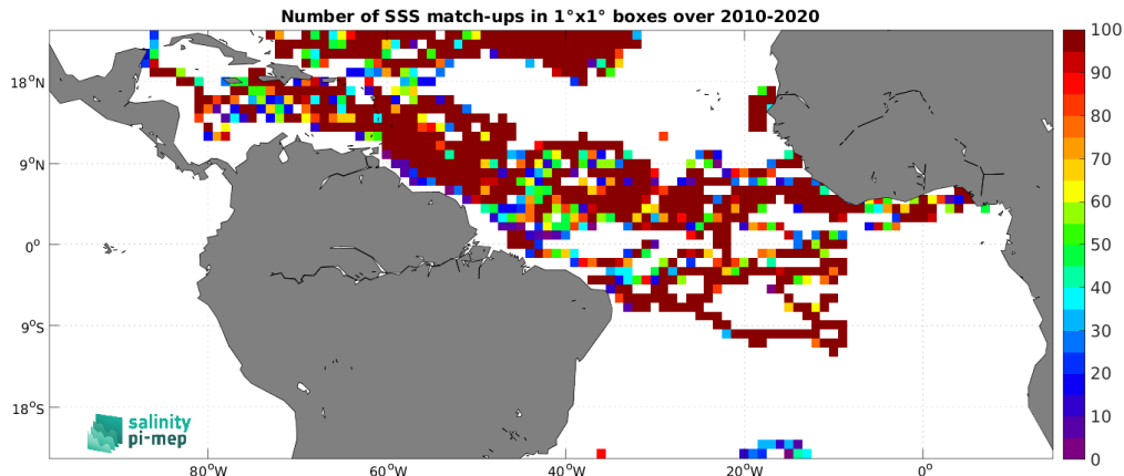
Figure 4: Number of SSS match-ups between Surface drifters SSS and the SMOS SSS L4 v1 - Monthly (CMEMS-CNR) SSS product for the Tropical Atlantic Ocean Pi-MEP region over 1^\circ \times 1^\circ boxes and for the full satellite product period.
