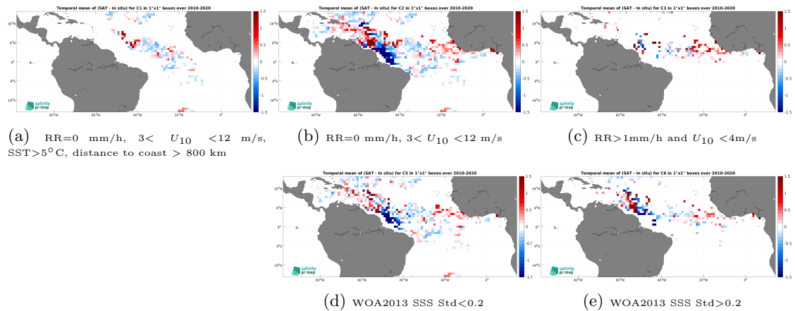
Figure 13: Temporal mean gridded over spatial boxes of size 1^\circ \times 1^\circ of \Delta\text{SSS} (SMOS SSS L4 v1 - Monthly (CMEMS-CNR) - Surface drifters) for 5 different subdatasets corresponding to:RR=0 mm/h, 3 < U_{10} < 12 m/s, SST >5^\circ\text{C} , distance to coast > 800 km (a), RR=0 mm/h, 3 < U_{10} < 12 m/s (b), RR >1 mm/h and U_{10} < 4 m/s (c), WOA2013 SSS Std <0.2 (d), WOA2013 SSS Std >0.2 (e).
