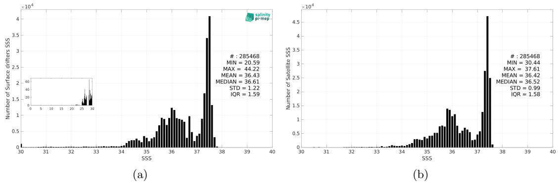
Figure 3: Histograms of SSS from Surface drifters (a) and SMOS SSS L4 v1 - Monthly (CMEMS-CNR) (b) considering all match-up pairs per bins of 0.1 over the Tropical Atlantic Ocean Pi-MEP region and for the full satellite product period.
