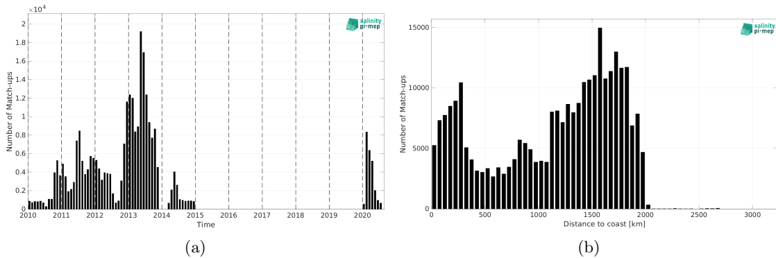
Figure 2: Number of match-ups between Surface drifters and SMOS SSS L4 v1 - Monthly (CMEMS-CNR) SSS as a function of time (a) and as function of the distance to coast (b) over the Tropical Atlantic Ocean Pi-MEP region and for the full satellite product period.
