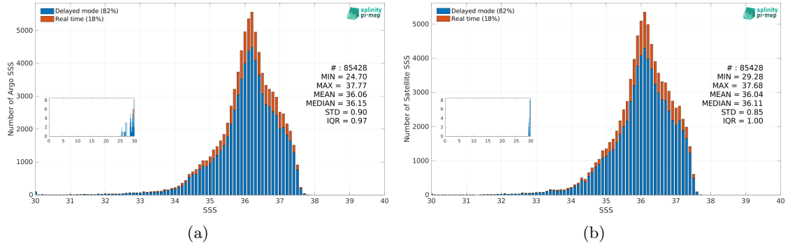
Figure 3: Histograms of SSS from Argo (a) and SMOS SSS L4 v1 - Monthly (CMEMS-CNR) (b) considering all match-up pairs per bins of 0.1 over the Tropical Atlantic Ocean Pi-MEP region and for the full satellite product period.
