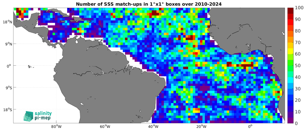
Figure 5: Number of SSS match-ups between Argo SSS and the SMOS SSS L4 v1 - Monthly (CMEMS-CNR) SSS product for the Tropical Atlantic Ocean Pi-MEP region over 1^\circ \times 1^\circ boxes and for the full satellite product period.
