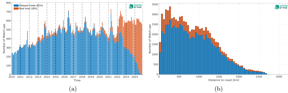
Figure 2: Number of match-ups between Argo and SMOS SSS L4 v1 - Monthly (CMEMS-CNR) SSS as a function of time (a) and as function of the distance to coast (b) over the Tropical Atlantic Ocean Pi-MEP region and for the full satellite product period.
