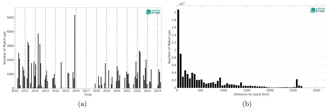
Figure 2: Number of match-ups between TSG (SAMOS) and SMOS SSS L4 v1 - Daily (CMEMS-CNR) SSS as a function of time (a) and as function of the distance to coast (b) over the Tropical Atlantic Ocean Pi-MEP region and for the full satellite product period.
