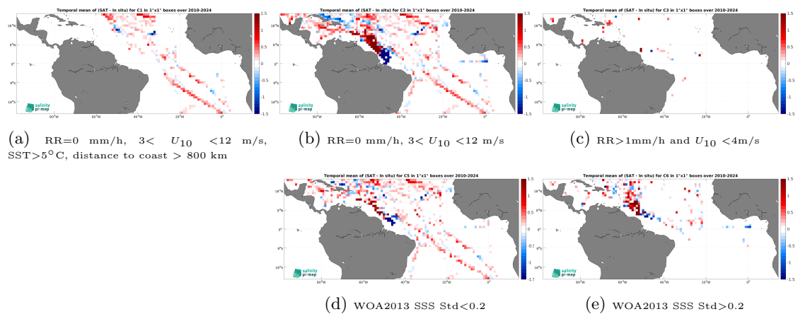
Figure 14: Temporal mean gridded over spatial boxes of size 1^\circ \times 1^\circ of \Delta\text{SSS} (SMOS SSS L4 v1 - Daily (CMEMS-CNR) - TSG (SAMOS)) for 5 different subdatasets corresponding to:RR=0 mm/h, 3 < U_{10} < 12 m/s, SST>5°C, distance to coast > 800 km (a), RR=0 mm/h, 3 < U_{10} < 12 m/s (b), RR>1mm/h and U_{10} < 4 m/s (c), WOA2013 SSS Std<0.2 (d), WOA2013 SSS Std>0.2 (e).
