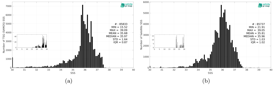
Figure 3: Histograms of SSS from TSG (SAMOS) (a) and SMOS SSS L4 v1 - Daily (CMEMS-CNR) (b) considering all match-up pairs per bins of 0.1 over the Tropical Atlantic Ocean Pi-MEP region and for the full satellite product period.
