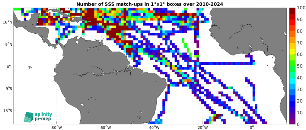
Figure 5: Number of SSS match-ups between TSG (SAMOS) SSS and the SMOS SSS L4 v1 - Daily (CMEMS-CNR) SSS product for the Tropical Atlantic Ocean Pi-MEP region over 1^\circ \times 1^\circ boxes and for the full satellite product period.
