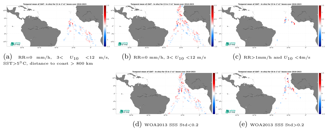
Figure 14: Temporal mean gridded over spatial boxes of size 1^\circ \times 1^\circ of \Delta\text{SSS} (SMOS SSS L4 v1 - Daily (CMEMS-CNR) - TSG (Polarstern)) for 5 different subdatasets corresponding to:RR=0 mm/h, 3 < U_{10} < 12 m/s, SST >5^\circ\text{C} , distance to coast > 800 km (a), RR=0 mm/h, 3 < U_{10} < 12 m/s (b), RR >1 mm/h and U_{10} < 4 m/s (c), WOA2013 SSS Std <0.2 (d), WOA2013 SSS Std >0.2 (e).
