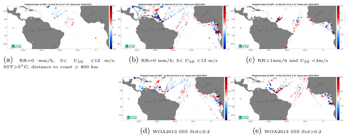
Figure 14: Temporal mean gridded over spatial boxes of size 1^\circ \times 1^\circ of \Delta\text{SSS} (SMOS SSS L4 v1 - Daily (CMEMS-CNR) - TSG (LEGOS-DM)) for 5 different subdatasets corresponding to:RR=0 mm/h, 3 < U_{10} < 12 m/s, SST >5^\circ\text{C} , distance to coast > 800 km (a), RR=0 mm/h, 3 < U_{10} < 12 m/s (b), RR >1 mm/h and U_{10} < 4 m/s (c), WOA2013 SSS Std <0.2 (d), WOA2013 SSS Std >0.2 (e).
