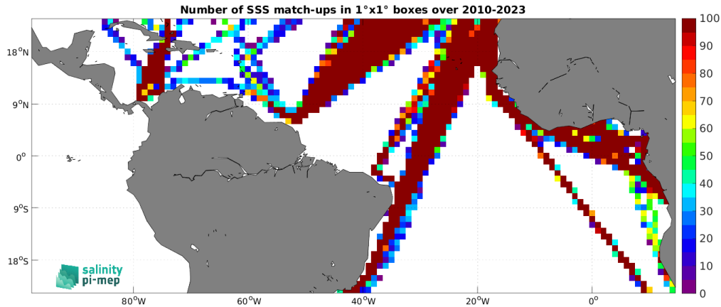
Figure 5: Number of SSS match-ups between TSG (LEGOS-DM) SSS and the SMOS SSS L4 v1 - Daily (CMEMS-CNR) SSS product for the Tropical Atlantic Ocean Pi-MEP region over 1^\circ \times 1^\circ boxes and for the full satellite product period.
