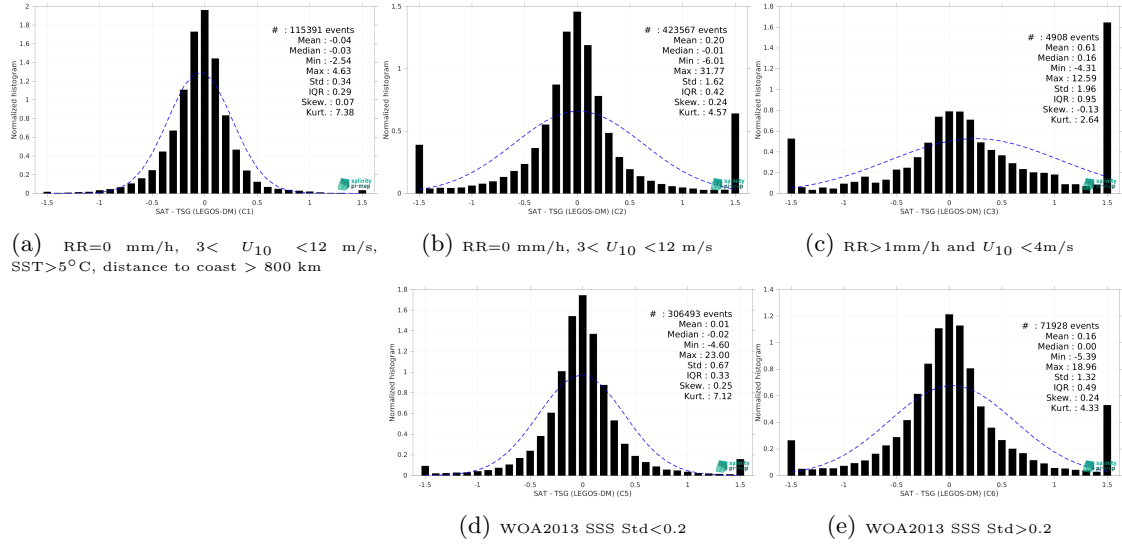
Figure 15: Normalized histogram of \Delta\text{SSS} (SMOS SSS L4 v1 - Daily (CMEMS-CNR) - TSG (LEGOS-DM)) for 5 different subdatasets corresponding to: RR=0 mm/h, 3 < U_{10} < 12 m/s, SST>5°C, distance to coast > 800 km (a), RR=0 mm/h, 3 < U_{10} < 12 m/s (b), RR>1mm/h and U_{10} < 4 m/s (c), WOA2013 SSS Std<0.2 (d), WOA2013 SSS Std>0.2 (e).
