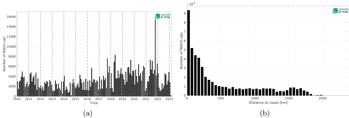
Figure 2: Number of match-ups between TSG (LEGOS-DM) and SMOS SSS L4 v1 - Daily (CMEMS-CNR) SSS as a function of time (a) and as function of the distance to coast (b) over the Tropical Atlantic Ocean Pi-MEP region and for the full satellite product period.
