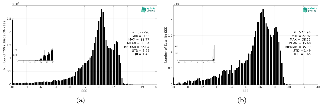
Figure 3: Histograms of SSS from TSG (LEGOS-DM) (a) and SMOS SSS L4 v1 - Daily (CMEMS-CNR) (b) considering all match-up pairs per bins of 0.1 over the Tropical Atlantic Ocean Pi-MEP region and for the full satellite product period.
